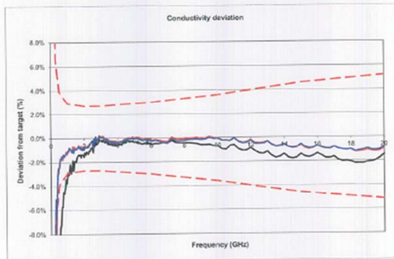
Fig. 3.2 Methanol conductivity deviation from target, 200 MHz – 20 GHz Conductivity error can be high at low frequencies due to the low absolute conductivity values.
