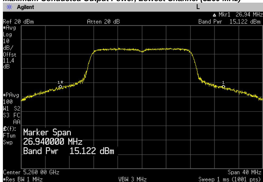
Maximum Conducted Output Power, Lowest Channel (5260 MHz)
