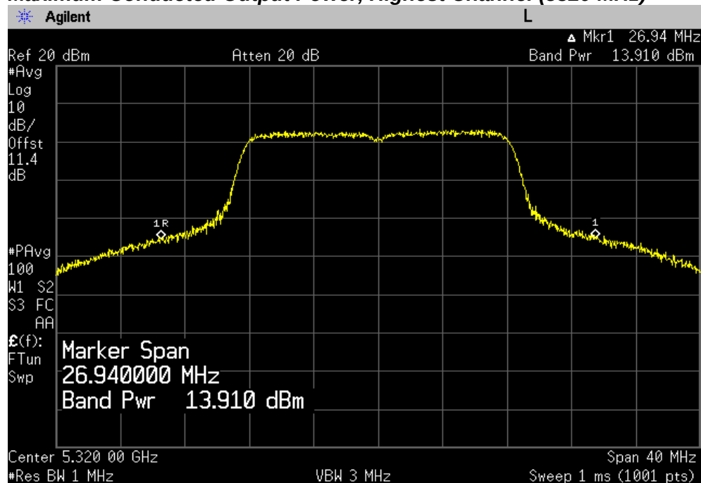
Maximum Conducted Output Power, Highest Channel (5320 MHz)
