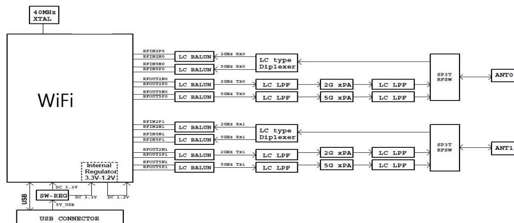
Figure 1-1 WiDT30Q Major Component and System Interface
