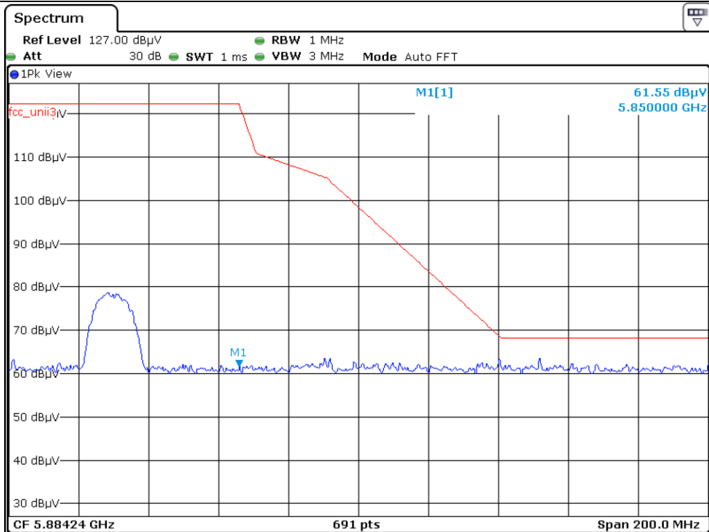
Middle Channel
