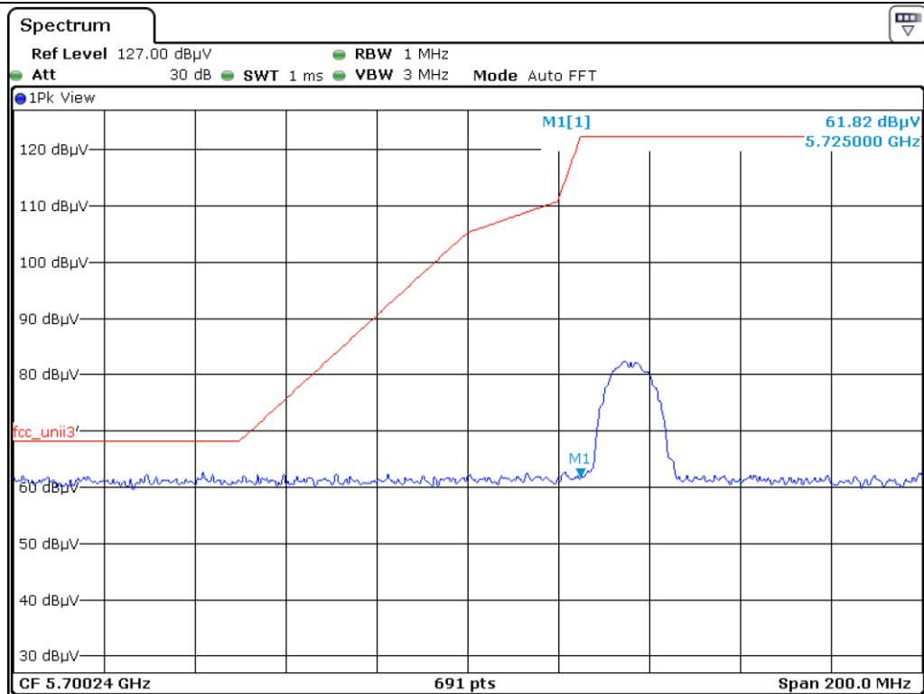
Low Channel
