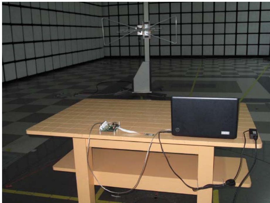
Radiated Test Picture(Rear)_ below 1G
