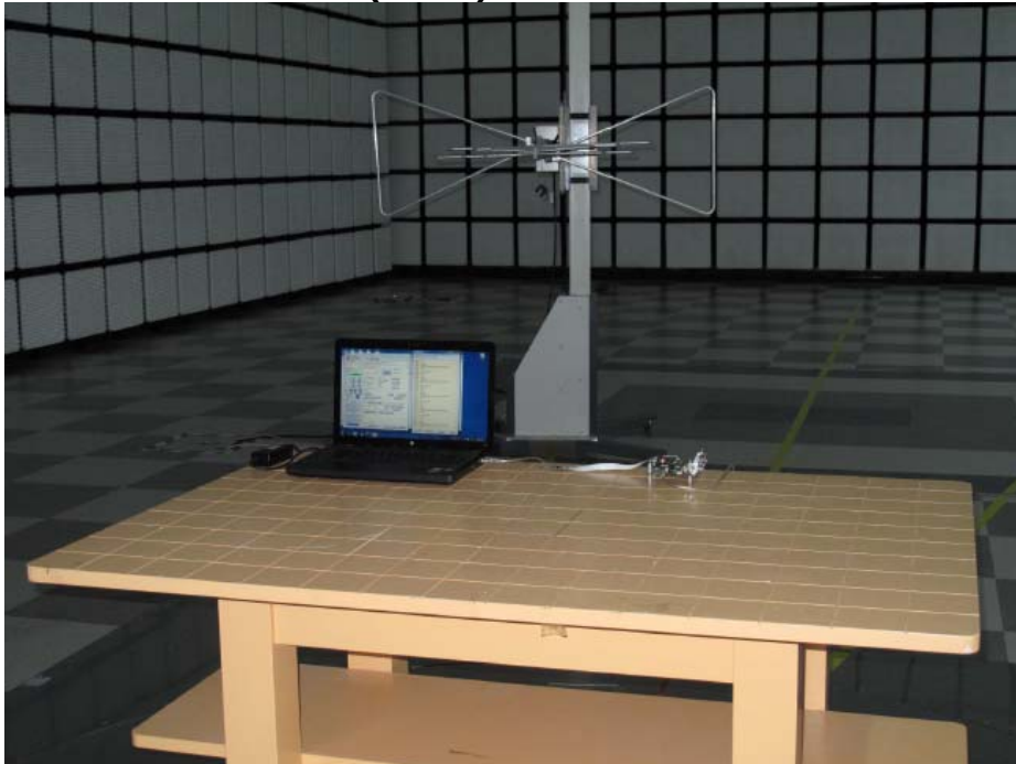
Radiated Test Picture(Front)_ below 1G
