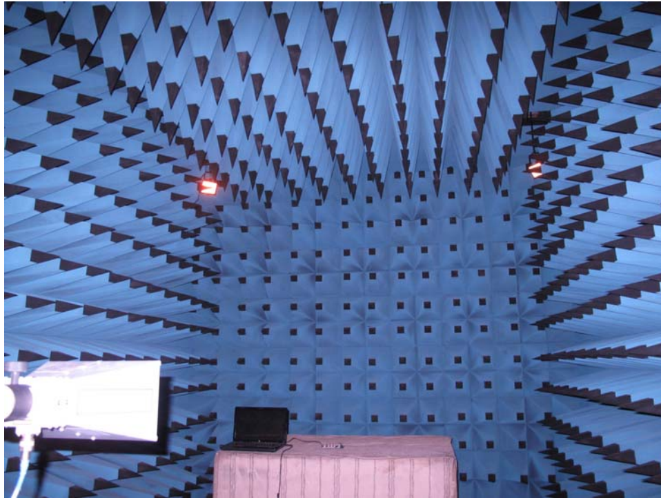
Radiated Test Picture(Front)_above 1G
