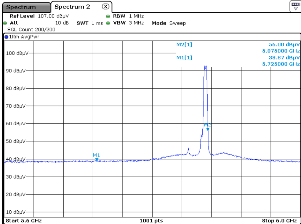
High Channel_Peak_V
