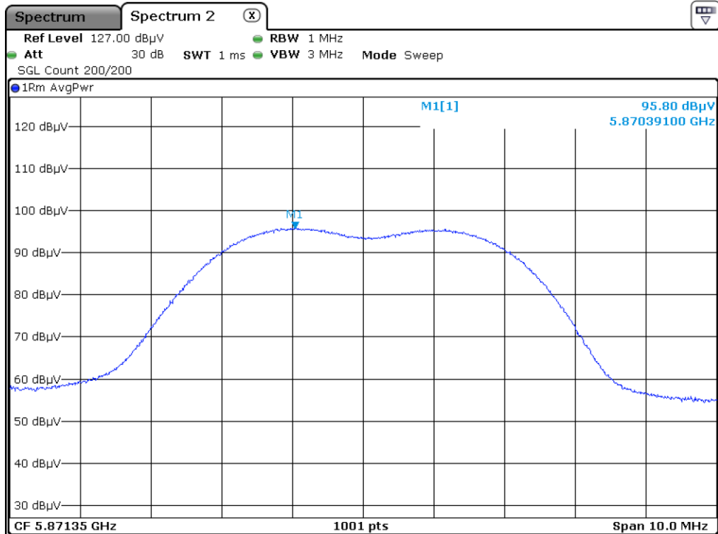
High Channel_Peak_H
