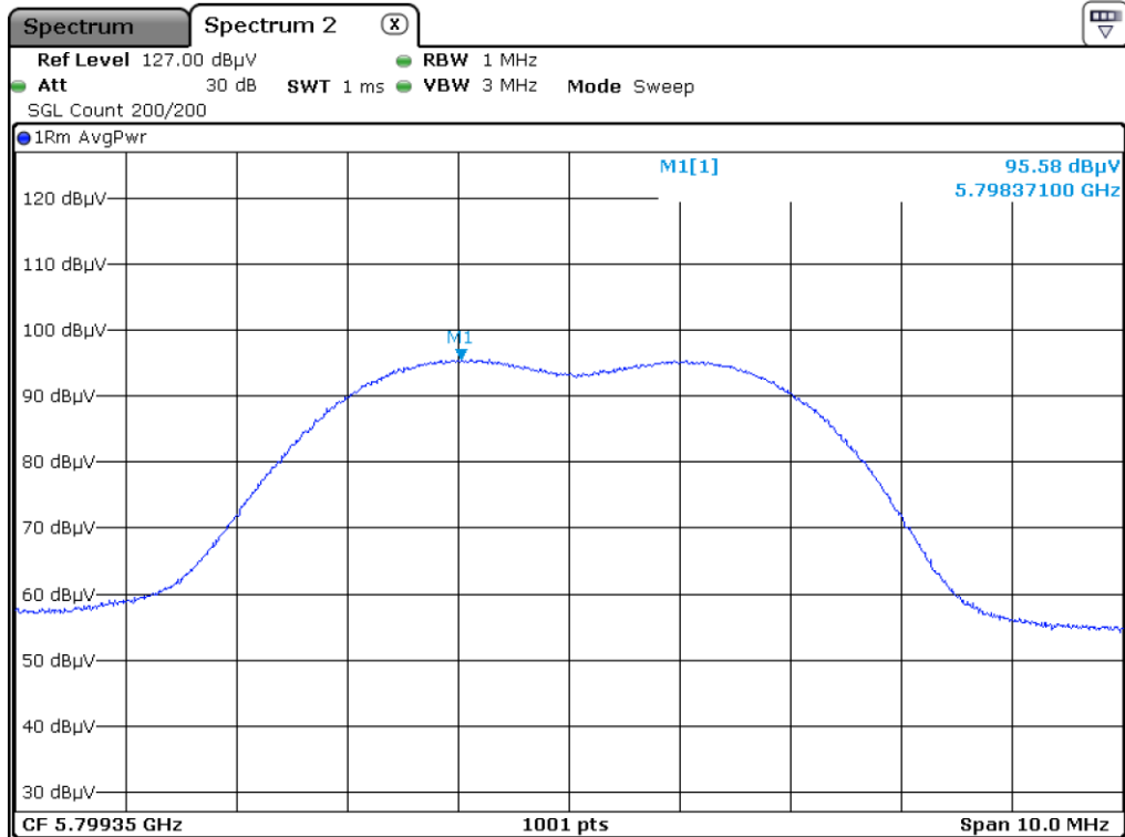
Middle Channel_Peak_V
