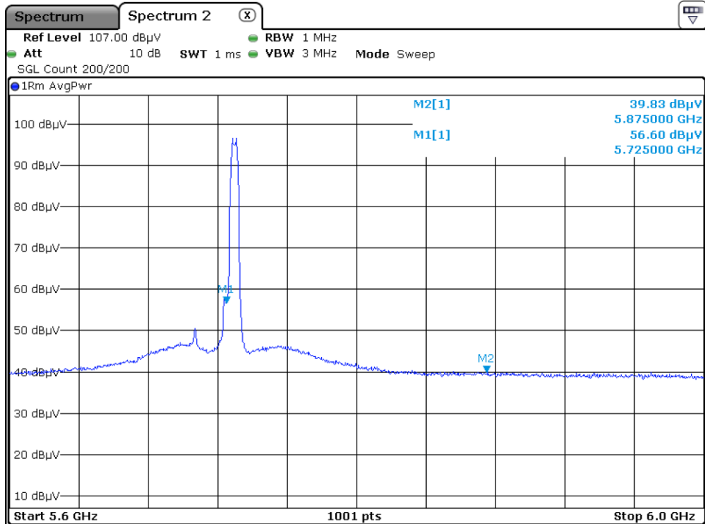
Low Channel_Peak_V
