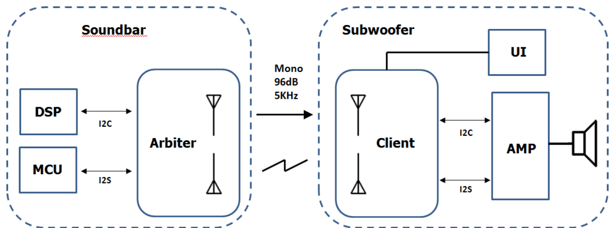
Wireless Subwoofer Solution Diagram
