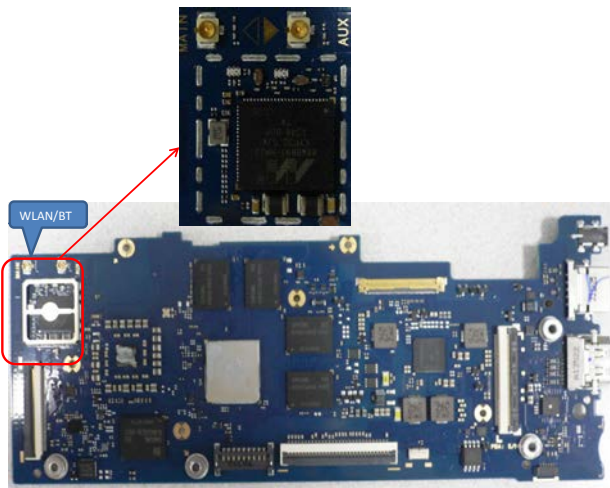
Main Board Top
