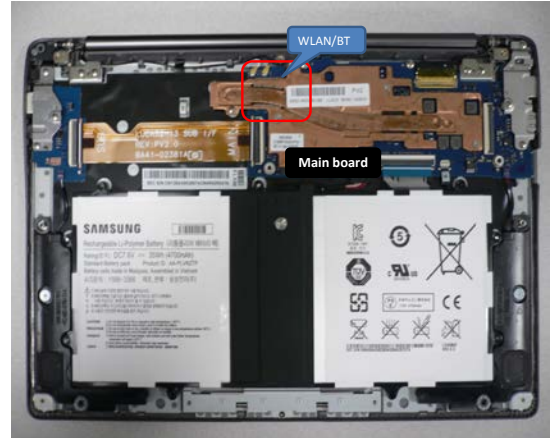
Main Board Bottom
