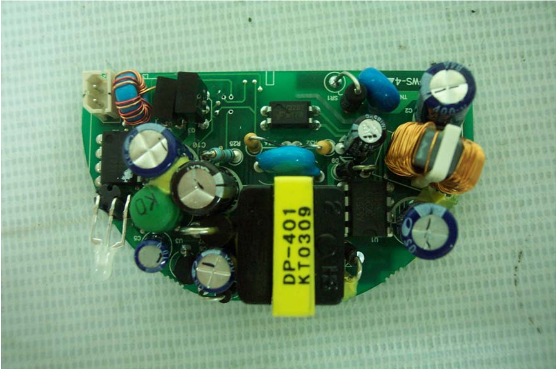
Adaptor pcb
