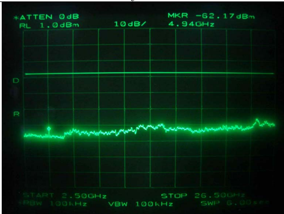
High Channel
