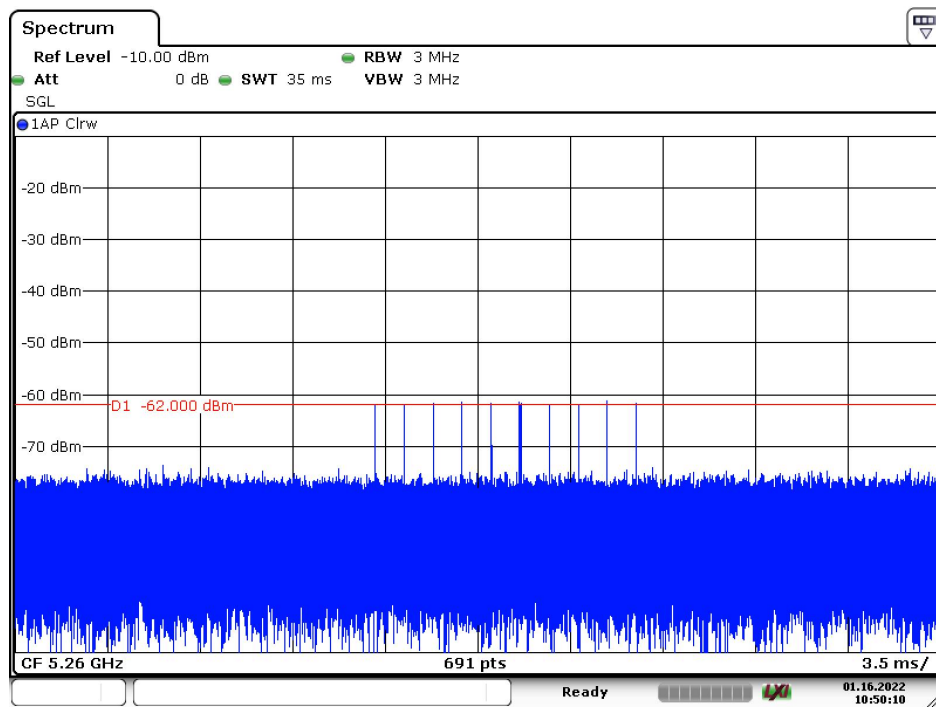
Radar Type 1B – 5260MHz
