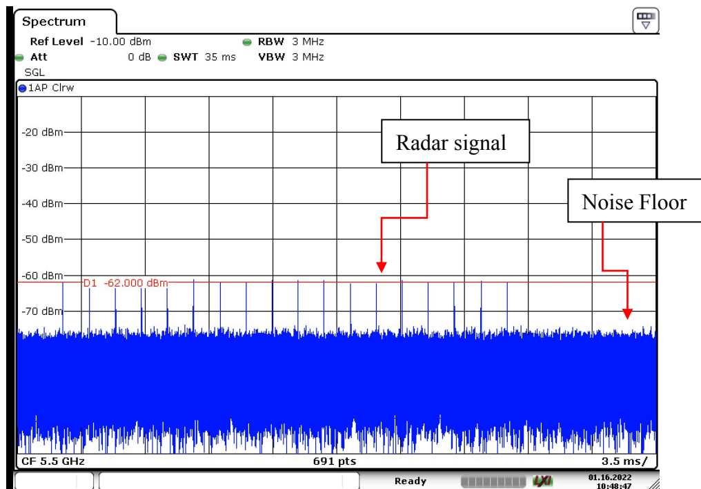
Radar Type 0 – 5500MHz
