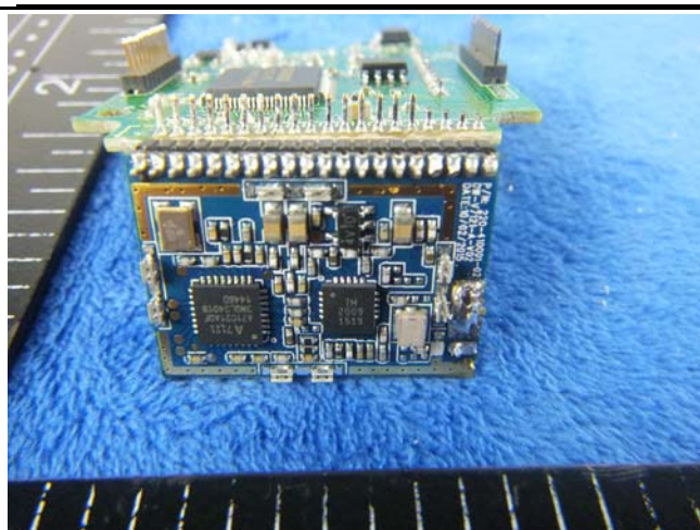
FHSS Board without shielding - Front View
