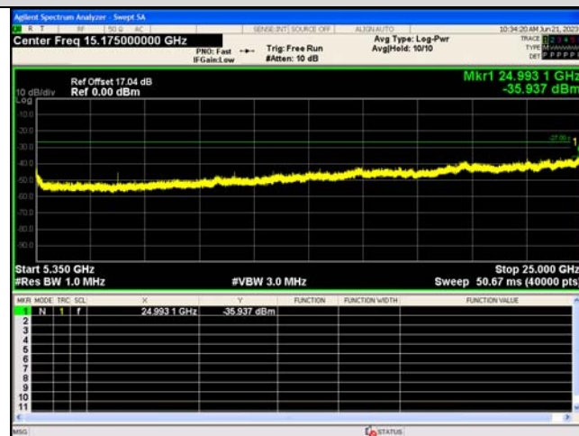
Spurious Emission:5350~25000.0 MHz IEEE 802.11ac_Channel 38_40MHz_Antenna 0
