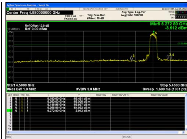
Out Of Band Emission IEEE 802.11ac_Channel 54_40MHz_Antenna 0
