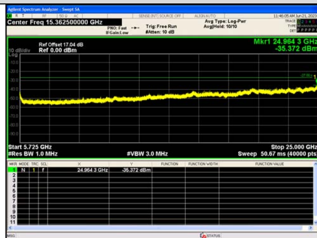
Spurious Emission:5725~25000.0 MHz IEEE 802.11ac_Channel 120_20MHz_Antenna 0
