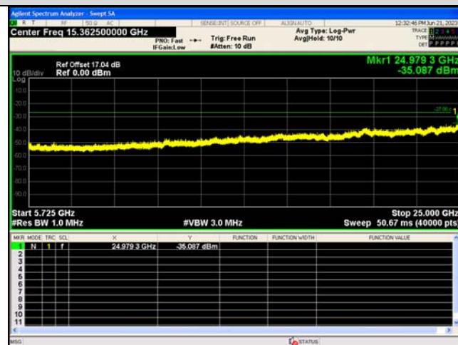
Spurious Emission:5725~25000.0 MHz IEEE 802.11ac_Channel 102_40MHz_Antenna 0
