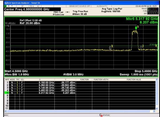
Out Of Band Emission IEEE 802.11n_Channel 62_40MHz_Antenna 0
