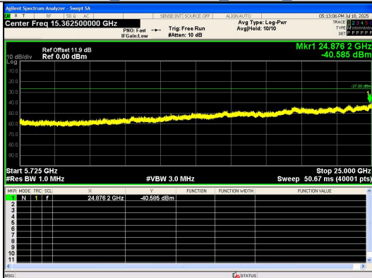
Spurious Emission:5725~25000.0 MHz IEEE 802.11n_Channel 102_40MHz_Antenna 0
