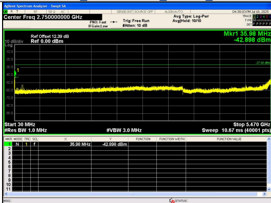
Spurious Emission:30.0~5470 MHz IEEE 802.11n_Channel 118_40MHz_Antenna 0
