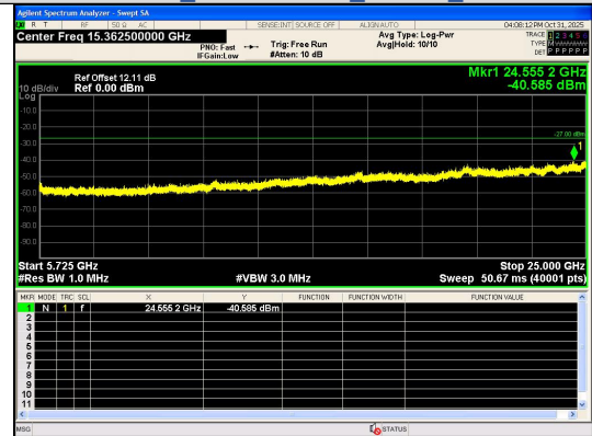
Spurious Emission:5725~25000.0 MHz IEEE 802.11n_Channel 100_20MHz_Antenna 0
