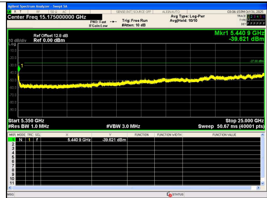
Spurious Emission:5350~25000.0 MHz IEEE 802.11n_Channel 56_20MHz_Antenna 0
