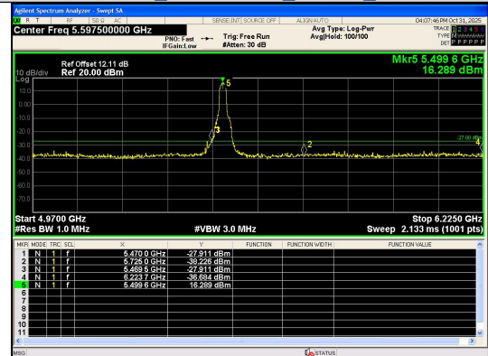
Out Of Band Emission IEEE 802.11n_Channel 100_20MHz_Antenna 0
