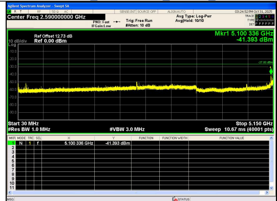
Spurious Emission:30.0~5150 MHz IEEE 802.11ac_Channel 52_20MHz_Antenna 0
