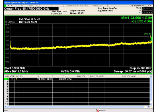
Spurious Emission:5350~25000.0 MHz IEEE 802.11ac_Channel 48_20MHz_Antenna 0
