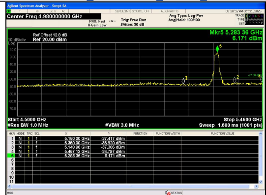
Out Of Band Emission IEEE 802.11ac_Channel 56_20MHz_Antenna 0
