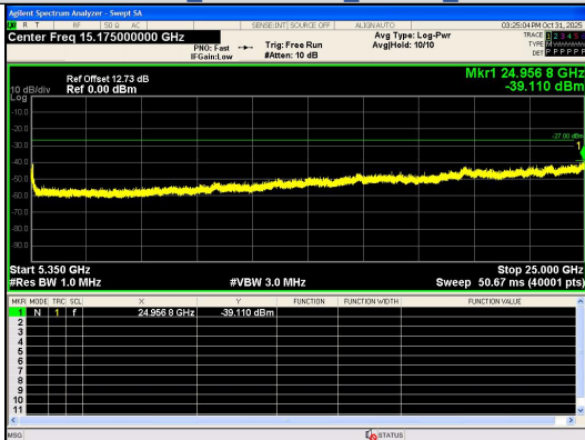
Spurious Emission:5350~25000.0 MHz IEEE 802.11ac_Channel 52_20MHz_Antenna 0
