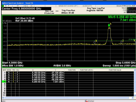
Out Of Band Emission IEEE 802.11ac_Channel 52_20MHz_Antenna 0
