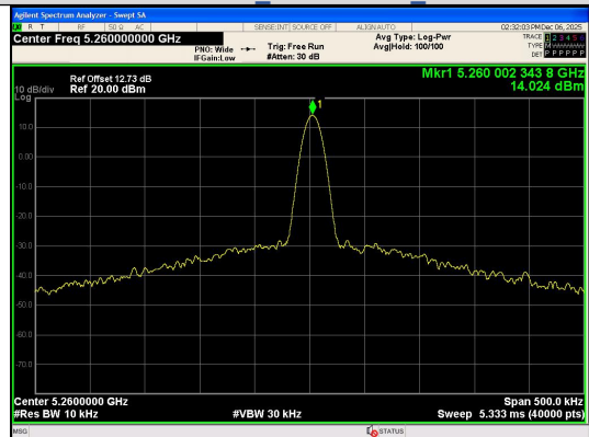
NT/NV_Antenna 0 IEEE 802.11a_Channel 52_20MHz
