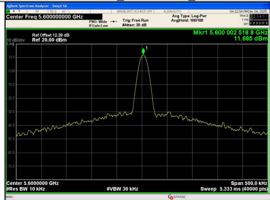
NT/NV_Antenna 0 IEEE 802.11a_Channel 120_20MHz
