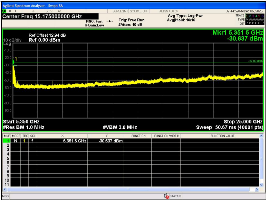
Spurious Emission:5350~25000.0 MHz IEEE 802.11a_Channel 64_20MHz_Antenna 0
