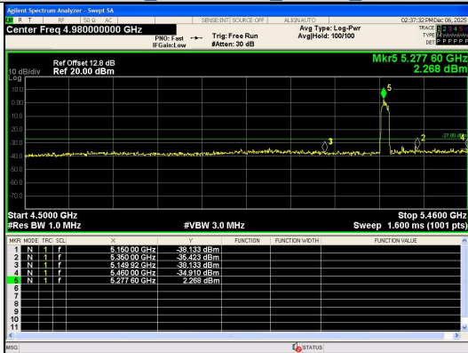
Out Of Band Emission IEEE 802.11a_Channel 56_20MHz_Antenna 0
