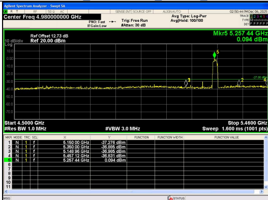
Out Of Band Emission IEEE 802.11n_Channel 52_20MHz_Antenna 0
