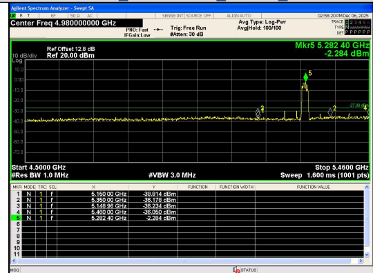
Out Of Band Emission IEEE 802.11n_Channel 56_20MHz_Antenna 0
