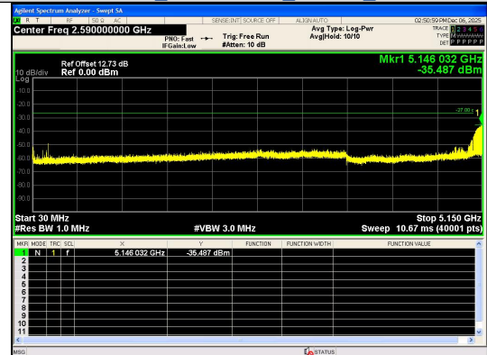
Spurious Emission:30.0~5150 MHz IEEE 802.11n_Channel 52_20MHz_Antenna 0
