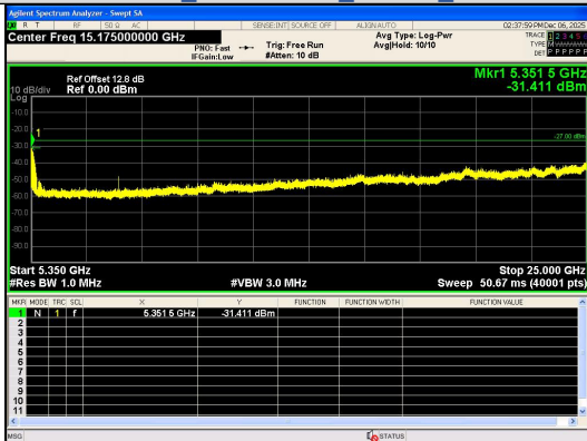
Spurious Emission:5350~25000.0 MHz IEEE 802.11a_Channel 56_20MHz_Antenna 0
