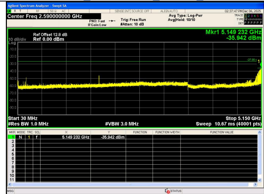
Spurious Emission:30.0~5150 MHz IEEE 802.11a_Channel 56_20MHz_Antenna 0
