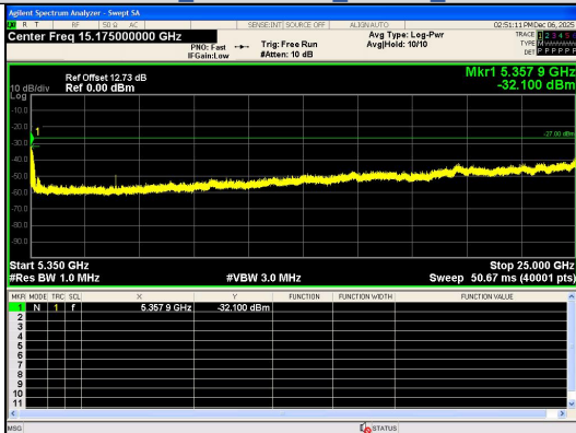
Spurious Emission:5350~25000.0 MHz IEEE 802.11n_Channel 52_20MHz_Antenna 0
