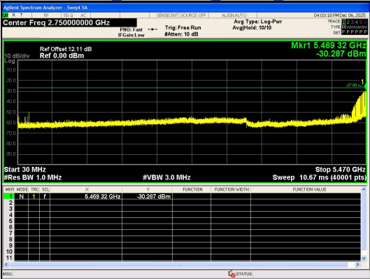
Spurious Emission:30.0~5470 MHz IEEE 802.11a_Channel 100_20MHz_Antenna 0
