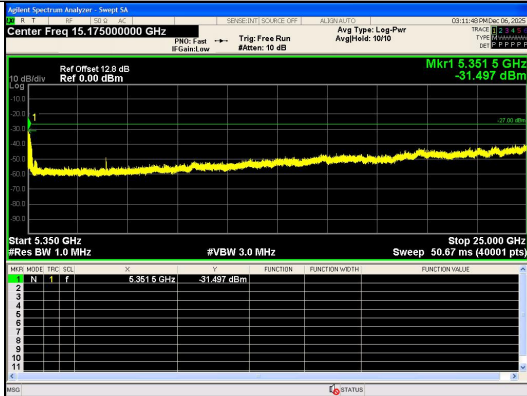
Spurious Emission:5350~25000.0 MHz IEEE 802.11n Channel 54 40MHz Antenna 0
