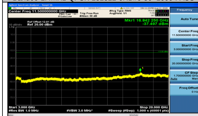
Band66-1.4MHz-QPSK-132322-6RB#0-3000~20000-PASS
