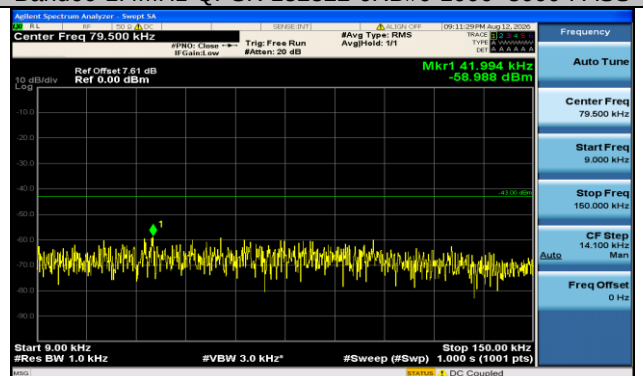
Band66-1.4MHz-16QAM-132322-6RB#0-0.009~0.15-PASS
