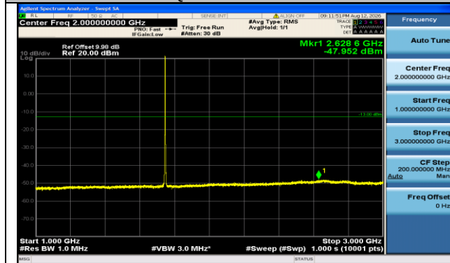
Band66-1.4MHz-16QAM-132322-6RB#0-1000~3000-PASS
