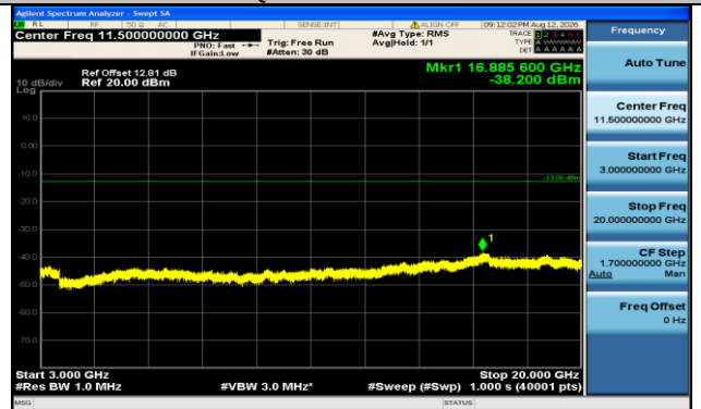
Band66-1.4MHz-16QAM-132322-6RB#0-3000~20000-PASS
