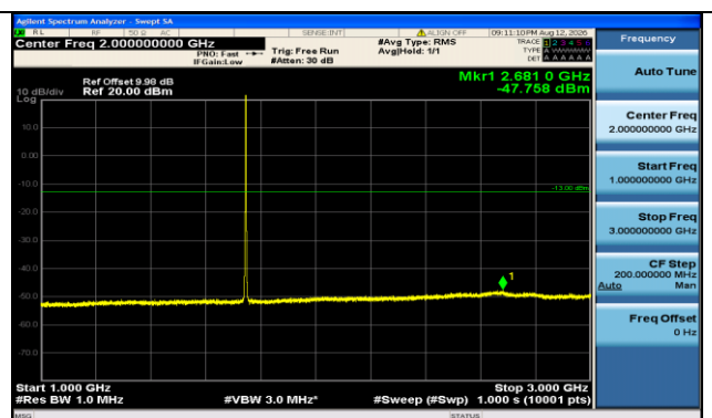
Band66-1.4MHz-OPSK-132322-6RB#0-1000~3000-PASS
