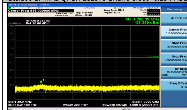
Band66-1.4MHz-QPSK-131979-1RB#0-30-1000-PASS
