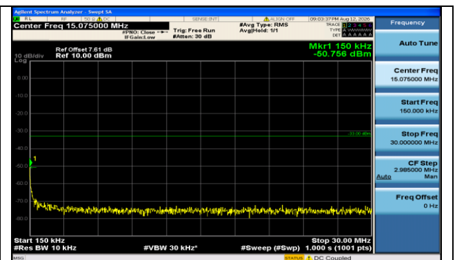
Band66-1.4MHz-QPSK-131979-1RB#0-0.15-30-PASS
