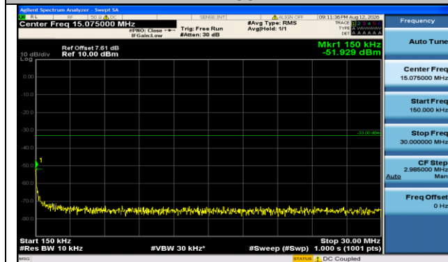
Band66-1.4MHz-16QAM-132322-6RB#0-0.15~30-PASS
