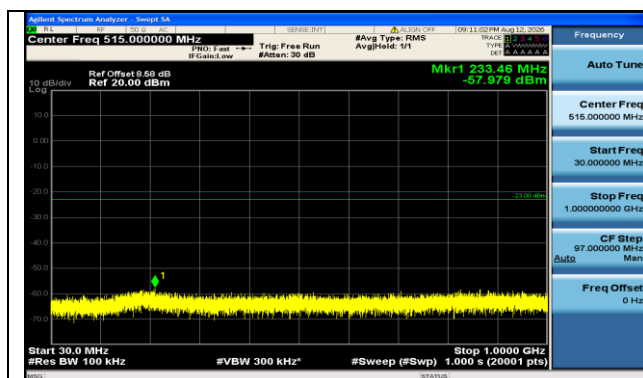
Band66-1.4MHz-OPSK-132322-6RB#0-30~1000-PASS
