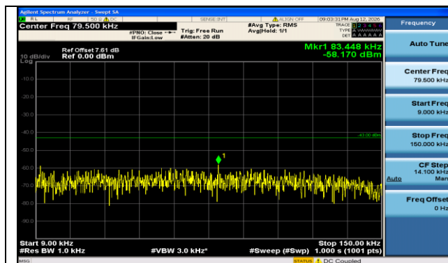
Band66-1.4MHz-QPSK-131979-1RB#0-0.009-0.15-PASS
