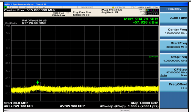
Band66-1.4MHz-16QAM-132322-6RB#0-30~1000-PASS
