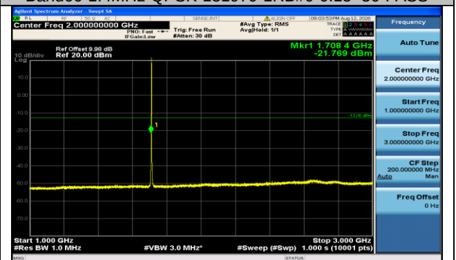
Band66-1.4MHz-QPSK-131979-1RB#0-1000-3000-PASS
