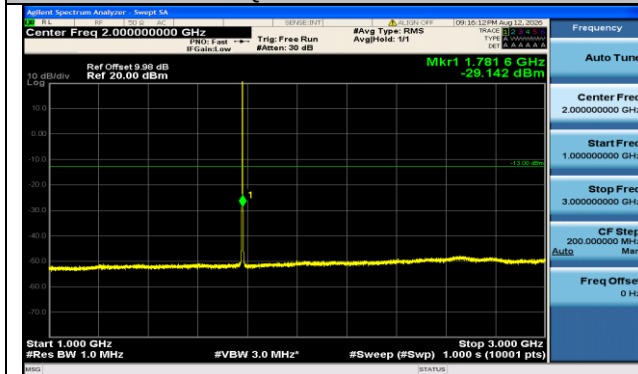
Band66-1.4MHz-16QAM-132665-6RB#0-1000~3000-PASS
