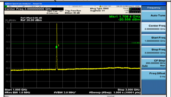
Band66-3MHz-QPSK-131987-15RB#0-1000~3000-PASS
