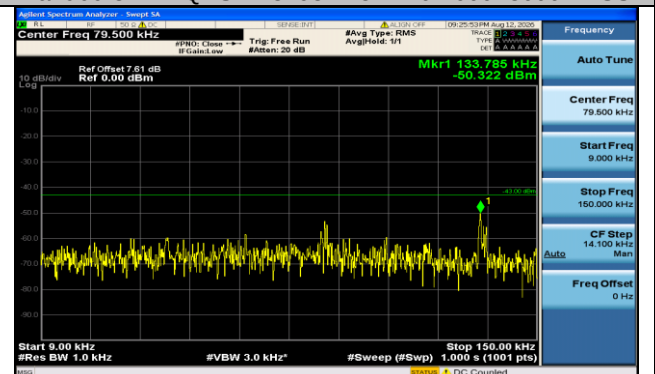
Band66-3MHz-16QAM-131987-15RB#0-0.009~0.15-PASS
