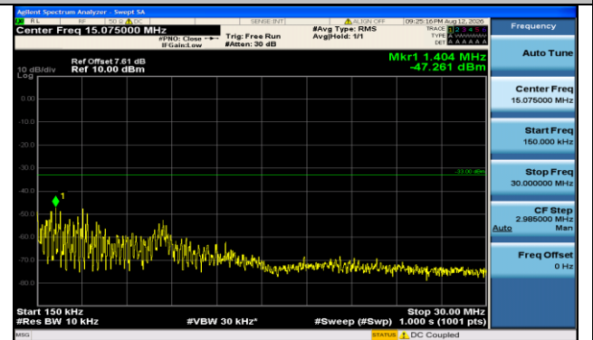
Band66-3MHz-QPSK-131987-15RB#0-0.15~30-PASS
