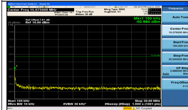
Band66-1.4MHz-16QAM-132665-6RB#0-0.15~30-PASS
