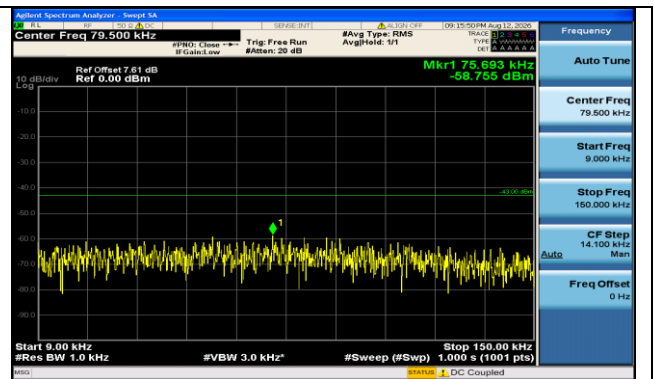
Band66-1.4MHz-16QAM-132665-6RB#0-0.009~0.15-PASS
