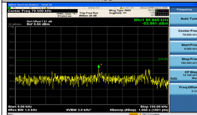
Band66-3MHz-QPSK-131987-1RB#0-0.009~0.15-PASS
