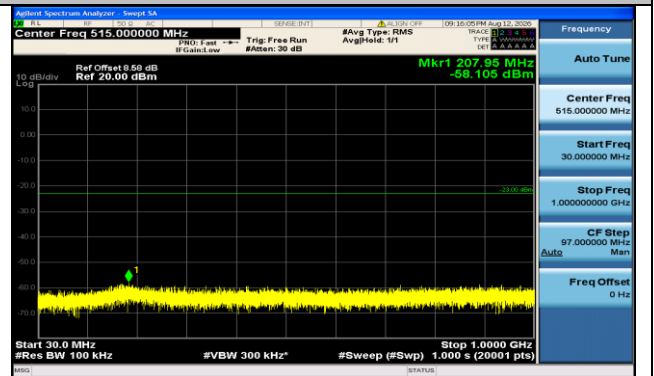
Band66-1.4MHz-16QAM-132665-6RB#0-30~1000-PASS
