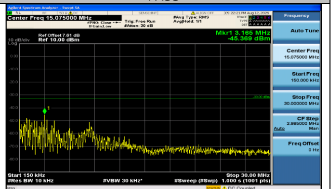
Band66-3MHz-QPSK-131987-1RB#0-0.15~30-PASS
