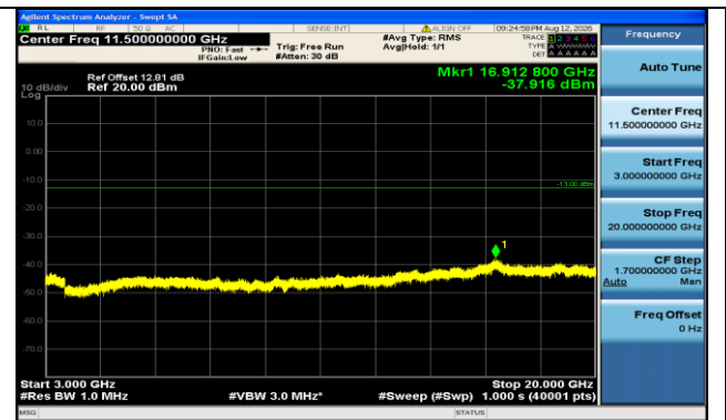
Band66-3MHz-16QAM-131987-1RB#14-3000~20000-PASS
