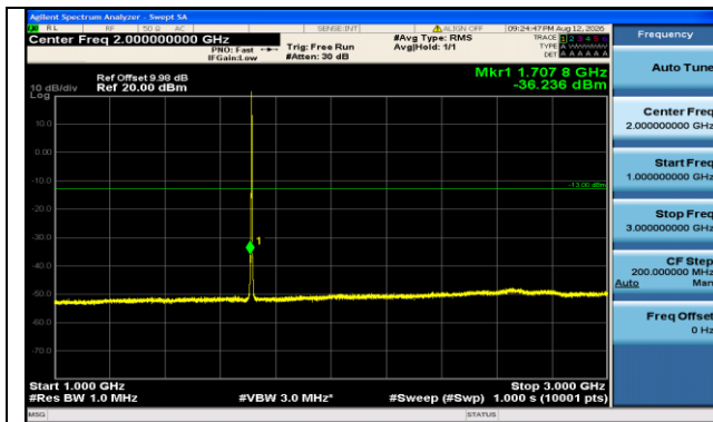
Band66-3MHz-16QAM-131987-1RB#14-1000~3000-PASS
