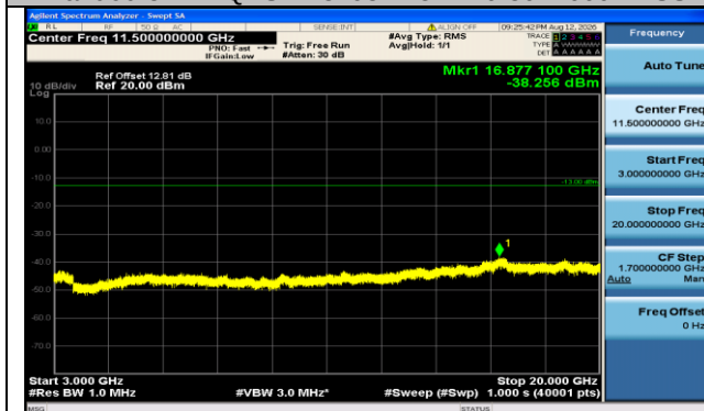
Band66-3MHz-QPSK-131987-15RB#0-3000~20000-PASS
