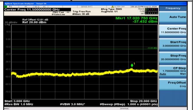
Band66-1.4MHz-16QAM-132665-6RB#0-3000~20000-PASS
