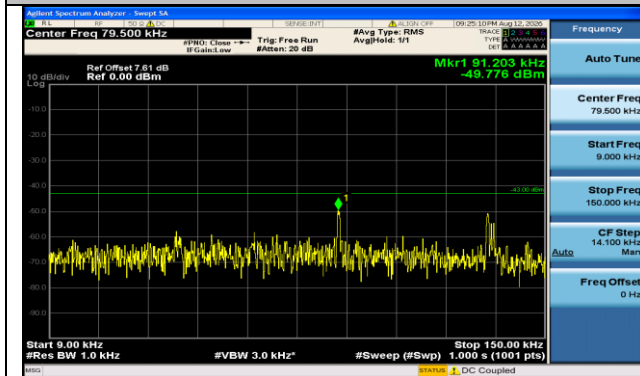
Band66-3MHz-QPSK-131987-15RB#0-0.009~0.15-PASS
