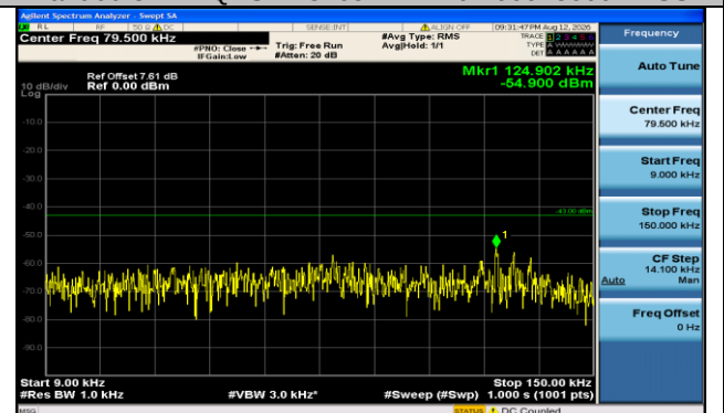
Band66-3MHz-16QAM-132657-1RB#0-0.009~0.15-PASS
