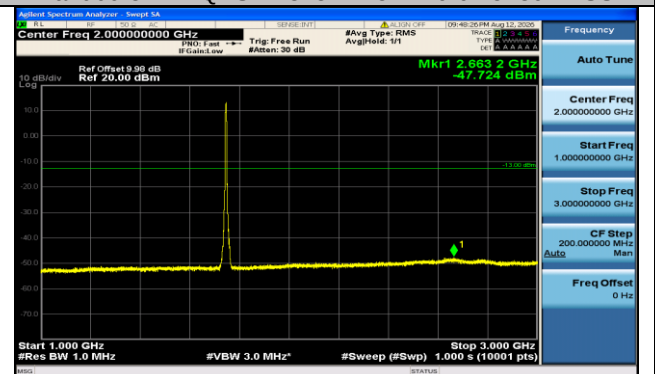
Band66-5MHz-QPSK-132322-25RB#0-1000~3000-PASS
