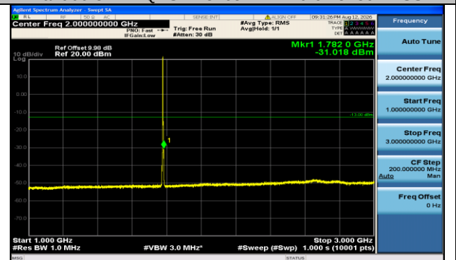
Band66-3MHz-QPSK-132657-1RB#0-1000~3000-PASS
