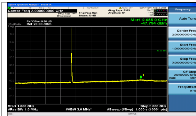
Band66-5MHz-16QAM-132322-1RB#24-1000~3000-PASS
