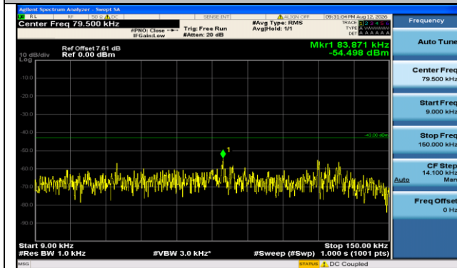
Band66-3MHz-QPSK-132657-1RB#0-0.009~0.15-PASS
