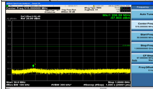
Band66-3MHz-QPSK-132657-1RB#0-30~1000-PASS
