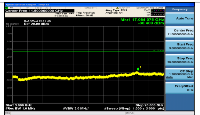
Band66-3MHz-16QAM-132322-15RB#0-3000~20000-PASS
