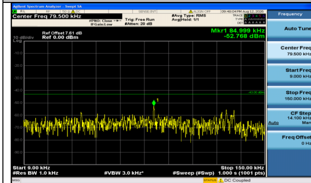
Band66-5MHz-QPSK-132322-25RB#0-0.009~0.15-PASS
