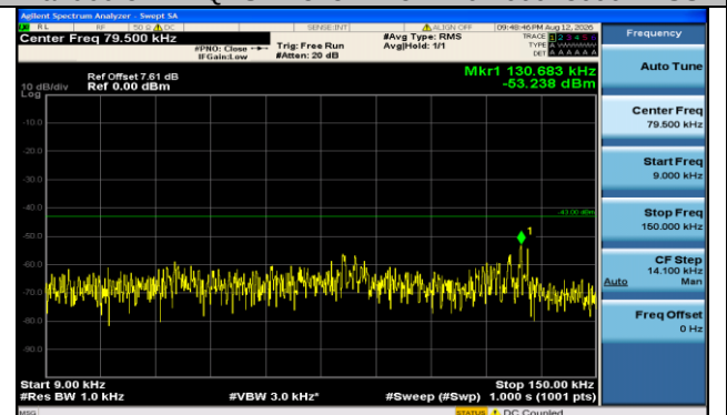
Band66-5MHz-16QAM-132322-25RB#0-0.009~0.15-PASS
