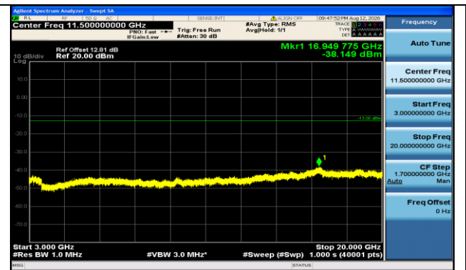
Band66-5MHz-16QAM-132322-1RB#24-3000~20000-PASS
