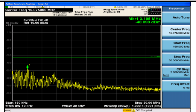
Band66-5MHz-QPSK-132322-25RB#0-0.15~30-PASS
