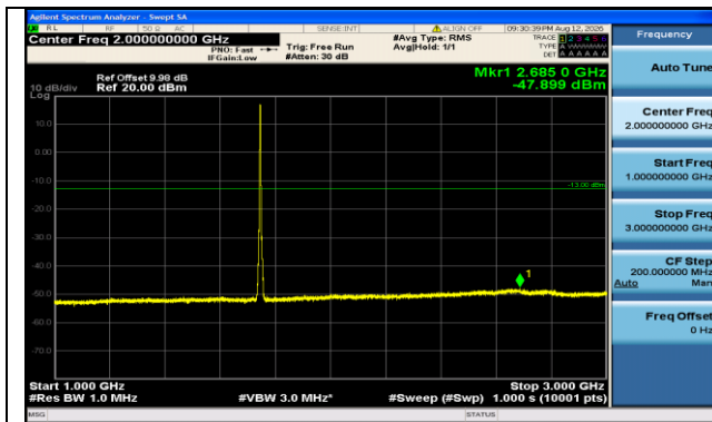
Band66-3MHz-16QAM-132322-15RB#0-1000~3000-PASS
