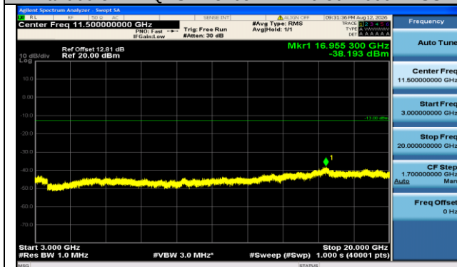
Band66-3MHz-QPSK-132657-1RB#0-3000~20000-PASS
