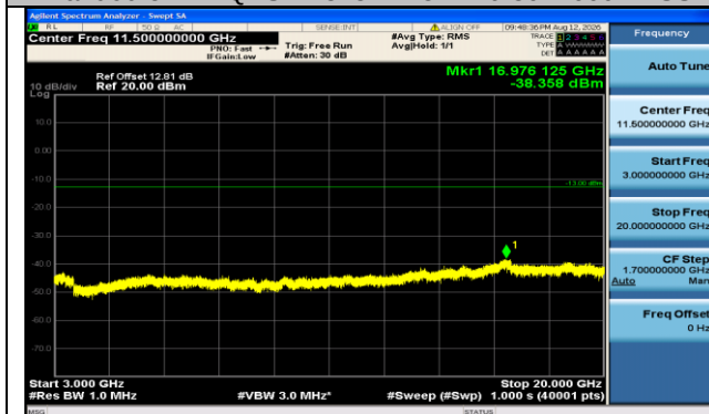
Band66-5MHz-QPSK-132322-25RB#0-3000~20000-PASS
