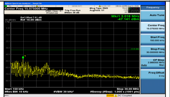
Band66-3MHz-QPSK-132657-1RB#0-0.15~30-PASS
