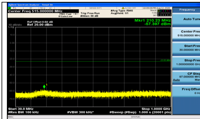
Band66-15MHz-16QAM-132047-1RB#74-30~1000-PASS
