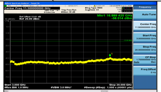
Band66-15MHz-QPSK-132047-75RB#0-3000~20000-PASS
