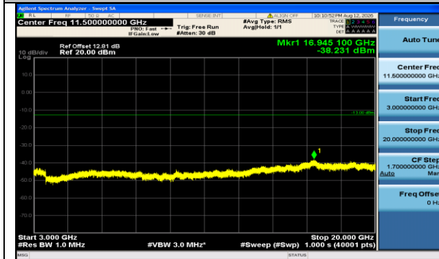
Band66-15MHz-16QAM-132047-75RB#0-3000~20000-PASS
