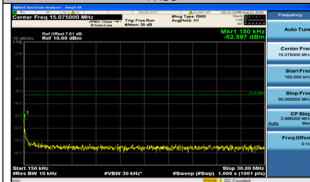
Band66-15MHz-QPSK-132322-1RB#0-0.15~30-PASS
