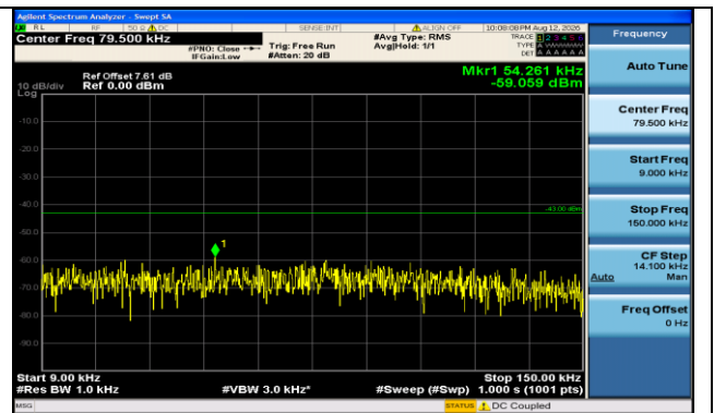
Band66-15MHz-QPSK-132047-1RB#74-0.009~0.15-PASS
