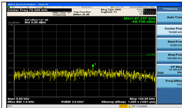
Band66-15MHz-16QAM-132047-75RB#0-0.009~0.15-PASS
