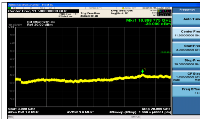
Band66-15MHz-16QAM-132047-1RB#0-3000~20000-PASS
