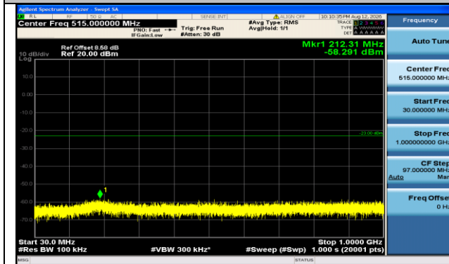
Band66-15MHz-16QAM-132047-75RB#0-30~1000-PASS
