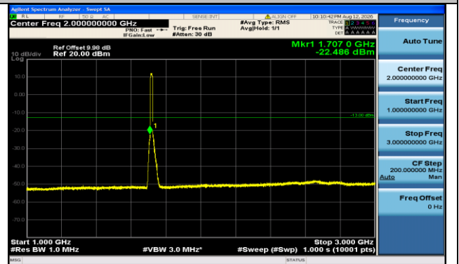
Band66-15MHz-16QAM-132047-75RB#0-1000~3000-PASS
