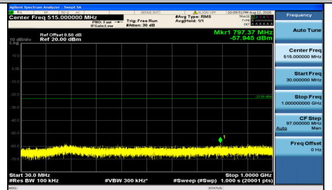
Band66-15MHz-QPSK-132047-75RB#0-30~1000-PASS
