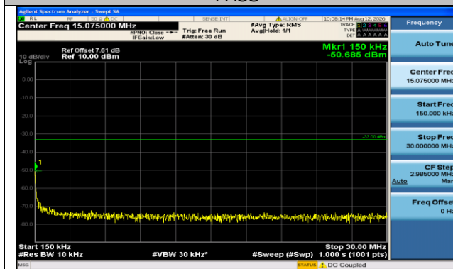
Band66-15MHz-QPSK-132047-1RB#74-0.15~30-PASS
