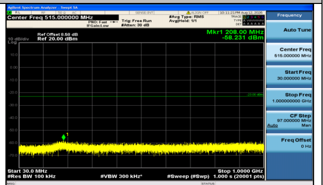
Band66-15MHz-QPSK-132322-1RB#0-30~1000-PASS
