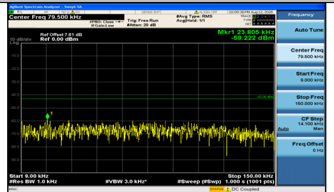
Band66-15MHz-QPSK-132047-75RB#0-0.009~0.15-PASS
