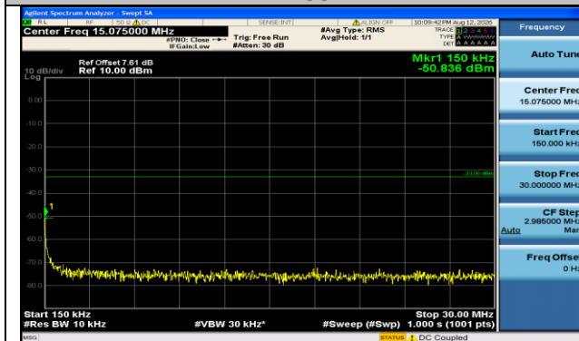
Band66-15MHz-QPSK-132047-75RB#0-0.15~30-PASS
