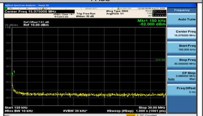
Band66-15MHz-16QAM-132047-1RB#74-0.15~30-PASS
