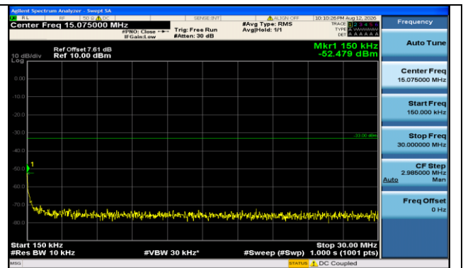
Band66-15MHz-16QAM-132047-75RB#0-0.15~30-PASS
