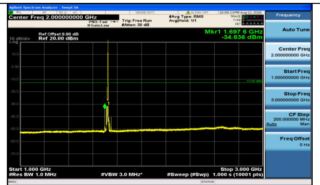
Band66-15MHz-16QAM-132047-1RB#74-1000~3000-PASS
