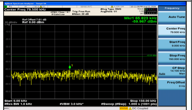
Band66-15MHz-QPSK-132322-1RB#0-0.009~0.15-PASS
