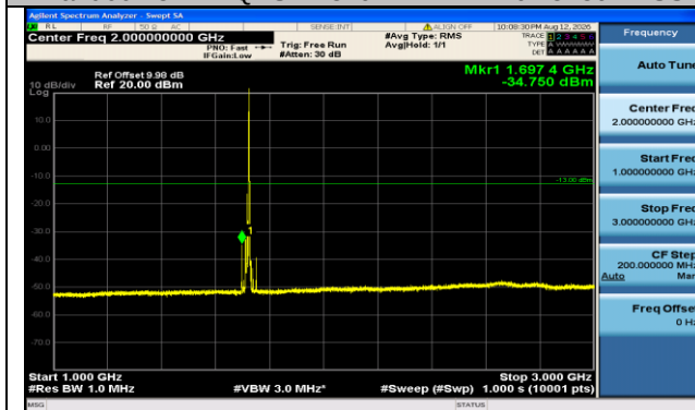
Band66-15MHz-QPSK-132047-1RB#74-1000~3000-PASS
