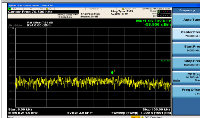
Band66-15MHz-16QAM-132047-1RB#74-0.009~0.15-PASS
