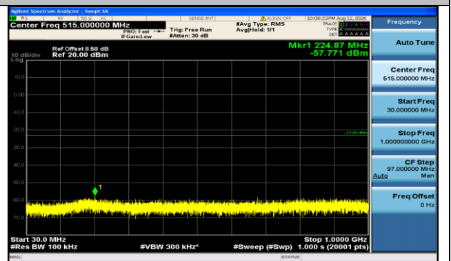
Band66-15MHz-QPSK-132047-1RB#74-30~1000-PASS
