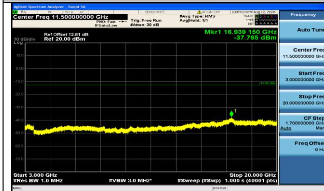
Band66-15MHz-16QAM-132047-1RB#74-3000~20000-PASS
