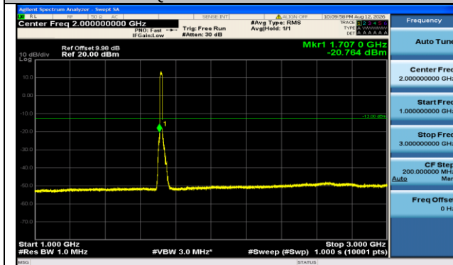
Band66-15MHz-QPSK-132047-75RB#0-1000~3000-PASS
