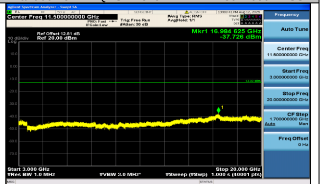
Band66-15MHz-QPSK-132047-1RB#74-3000~20000-PASS
