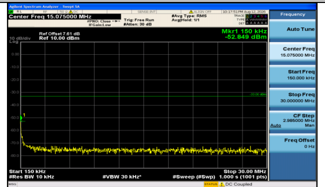
Band66-15MHz-16QAM-132597-1RB#74-0.15~30-PASS
