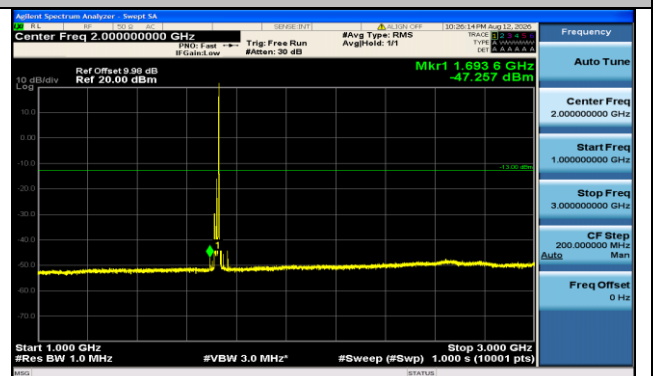
Band66-20MHz-16QAM-132072-1RB#99-1000~3000-PASS
