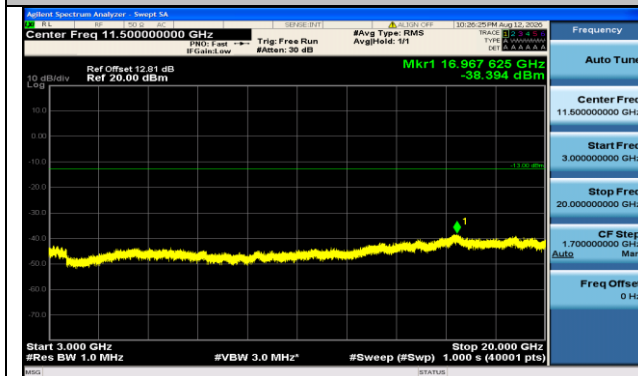
Band66-20MHz-16QAM-132072-1RB#99-3000~20000-PASS
