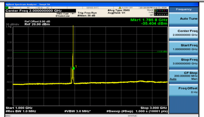
Band66-15MHz-16QAM-132597-1RB#74-1000~3000-PASS
