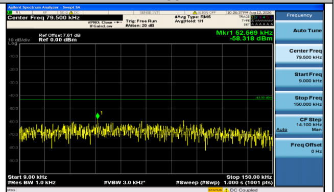
Band66-20MHz-QPSK-132072-100RB#0-0.009~0.15-PASS
