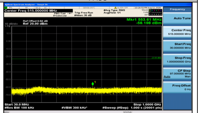
Band66-20MHz-QPSK-132072-100RB#0-30~1000-PASS
