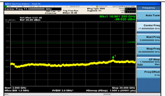
Band66-15MHz-QPSK-132597-1RB#74-3000~20000-PASS
