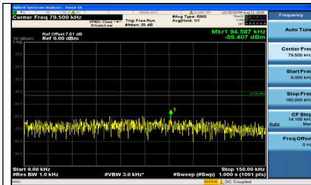
Band66-20MHz-16QAM-132072-1RB#99-0.009~0.15-PASS
