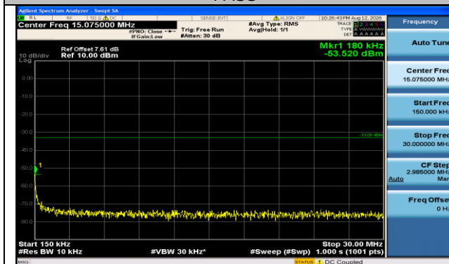
Band66-20MHz-QPSK-132072-100RB#0-0.15~30-PASS
