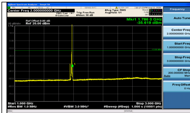
Band66-15MHz-QPSK-132597-1RB#74-1000~3000-PASS
