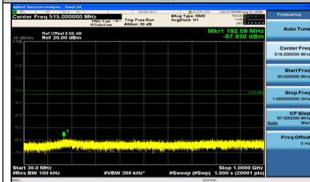
Band66-15MHz-16QAM-132597-1RB#74-30~1000-PASS
