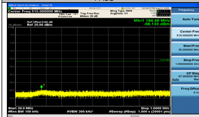
Band66-20MHz-16QAM-132072-1RB#99-30~1000-PASS
