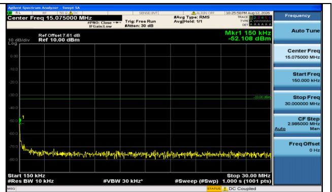
Band66-20MHz-16QAM-132072-1RB#99-0.15~30-PASS
