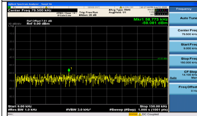
Band66-15MHz-16QAM-132597-1RB#74-0.009~0.15-PASS
