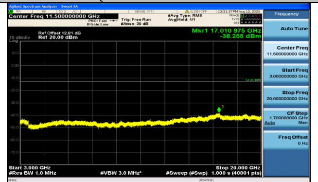
Band66-20MHz-QPSK-132322-100RB#0-3000~20000-PASS
