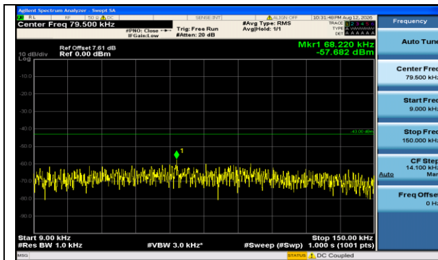
Band66-20MHz-16QAM-132322-100RB#0-0.009~0.15-PASS
