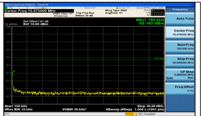
Band66-20MHz-16QAM-132322-100RB#0-0.15~30-PASS
