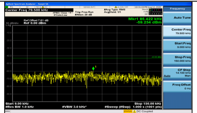
Band66-20MHz-QPSK-132322-100RB#0-0.009~0.15-PASS
