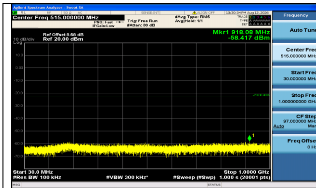
Band66-20MHz-16QAM-132322-1RB#99-30~1000-PASS
