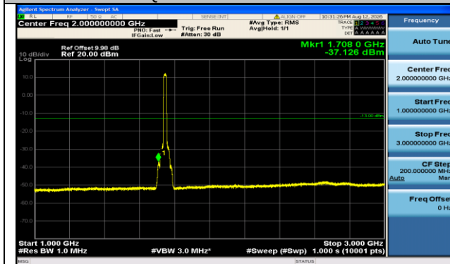
Band66-20MHz-QPSK-132322-100RB#0-1000~3000-PASS
