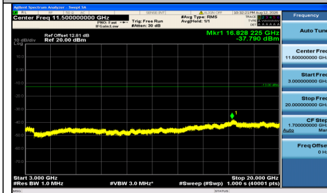
Band66-20MHz-16QAM-132322-100RB#0-3000~20000-PASS
