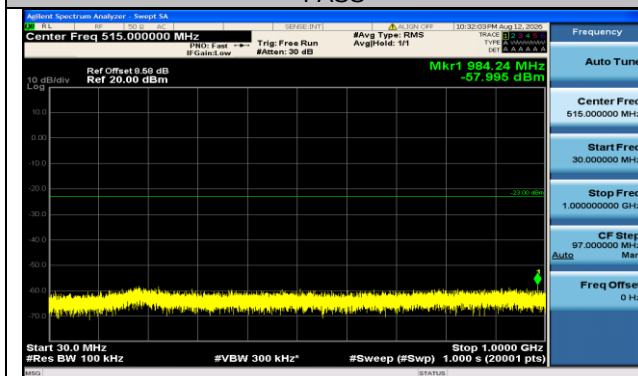
Band66-20MHz-16QAM-132322-100RB#0-30~1000-PASS
