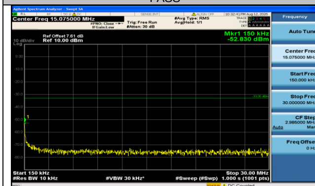
Band66-20MHz-QPSK-132572-1RB#0-0.15~30-PASS
