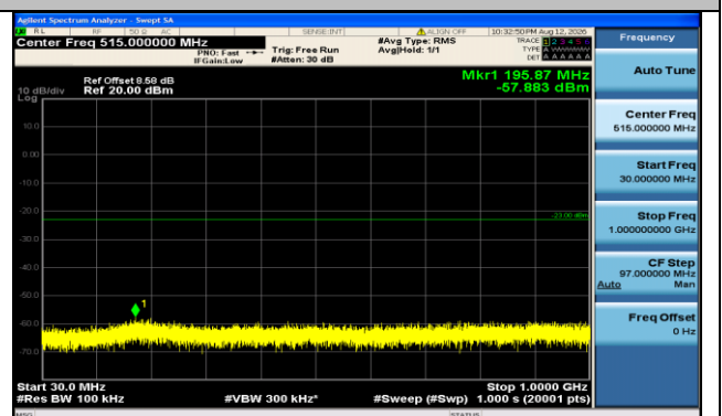
Band66-20MHz-QPSK-132572-1RB#0-30~1000-PASS
