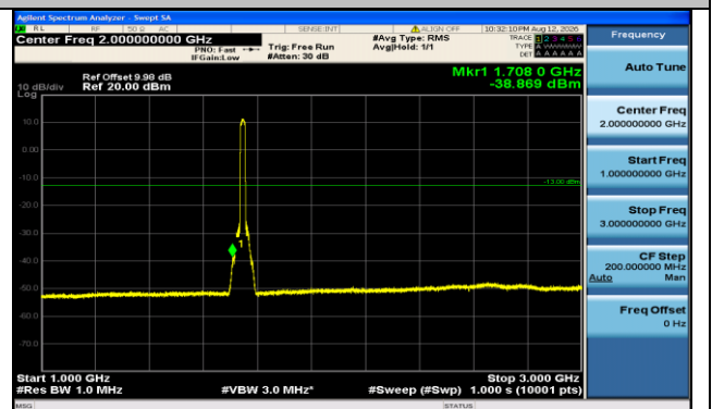
Band66-20MHz-16QAM-132322-100RB#0-1000~3000-PASS
