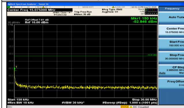
Band66-20MHz-QPSK-132322-100RB#0-0.15~30-PASS
