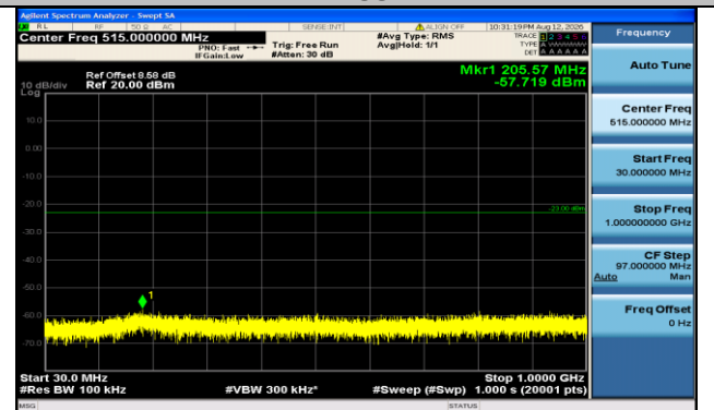
Band66-20MHz-QPSK-132322-100RB#0-30~1000-PASS
