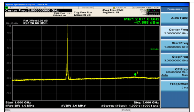
Band66-20MHz-16QAM-132322-1RB#99-1000~3000-PASS
