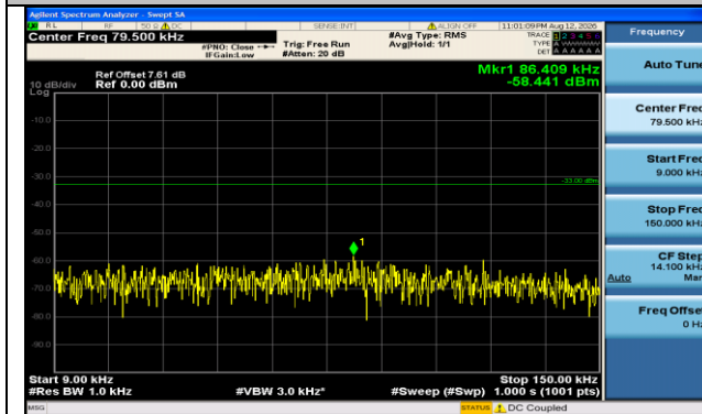
Band71-10MHz-QPSK-133172-1RB#49-0.009~0.15-PASS
