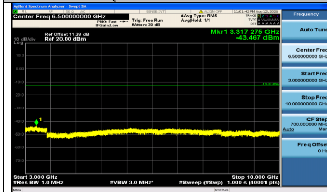
Band71-10MHz-QPSK-133172-1RB#49-3000~10000-PASS
