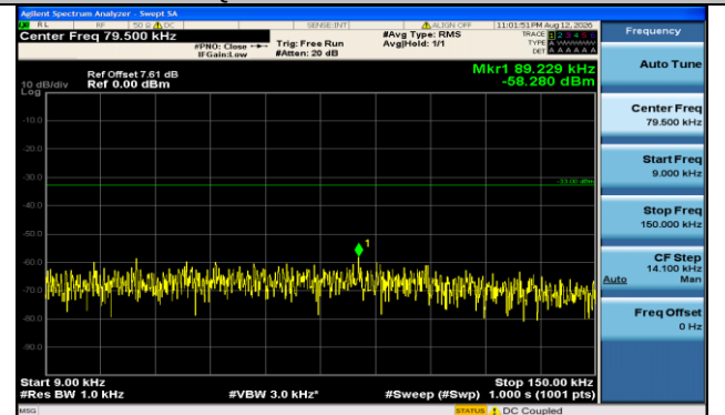
Band71-10MHz-16QAM-133172-1RB#49-0.009~0.15-PASS
