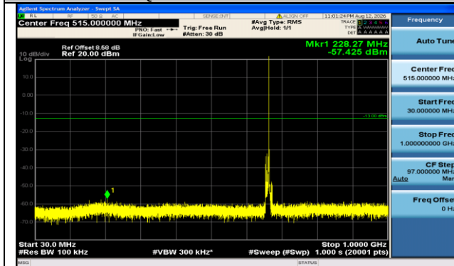
Band71-10MHz-QPSK-133172-1RB#49-30~1000-PASS
