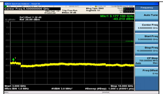
Band71-10MHz-16QAM-133172-1RB#0-3000~10000-PASS
