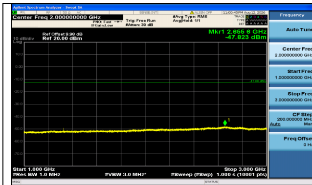
Band71-10MHz-16QAM-133172-1RB#0-1000~3000-PASS
