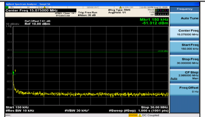
Band71-10MHz-QPSK-133172-1RB#49-0.15~30-PASS
