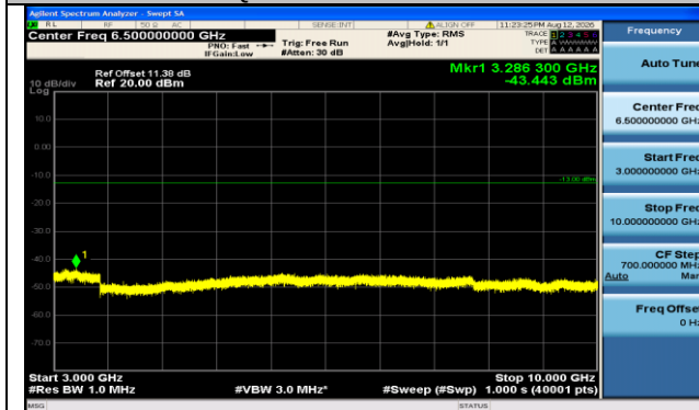
Band71-15MHz-QPSK-133297-1RB#74-3000~10000-PASS
