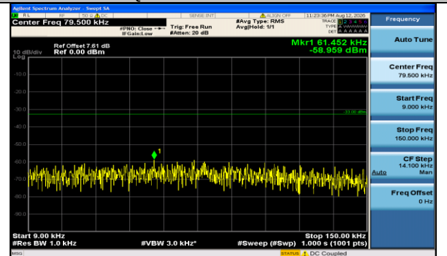
Band71-15MHz-16QAM-133297-1RB#74-0.009~0.15-PASS
