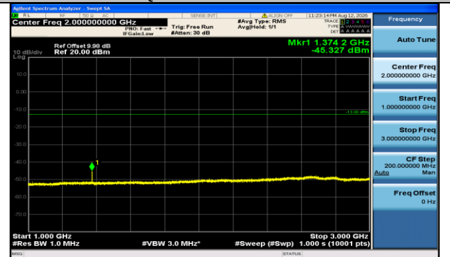
Band71-15MHz-QPSK-133297-1RB#74-1000~3000-PASS
