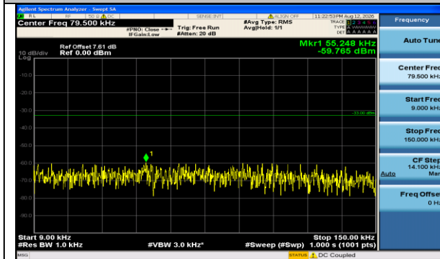
Band71-15MHz-QPSK-133297-1RB#74-0.009~0.15-PASS
