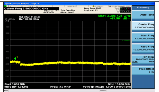
Band71-15MHz-16QAM-133297-1RB#0-3000~10000-PASS
