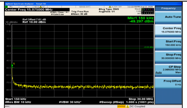
Band71-15MHz-QPSK-133297-1RB#74-0.15~30-PASS
