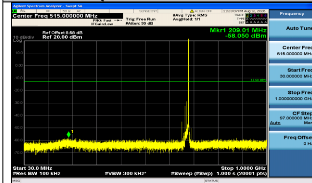
Band71-15MHz-QPSK-133297-1RB#74-30~1000-PASS
