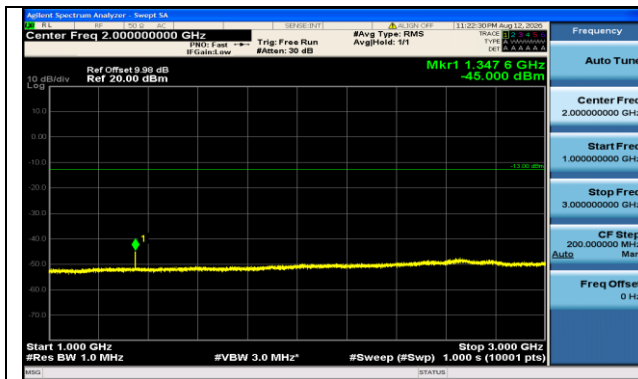
Band71-15MHz-16QAM-133297-1RB#0-1000~3000-PASS
