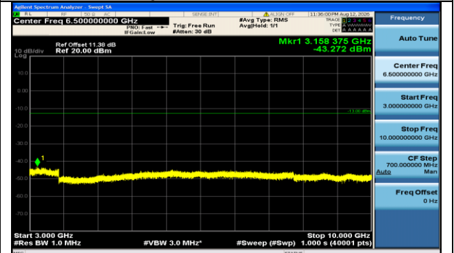
Band71-20MHz-QPSK-133222-1RB#99-3000~10000-PASS
