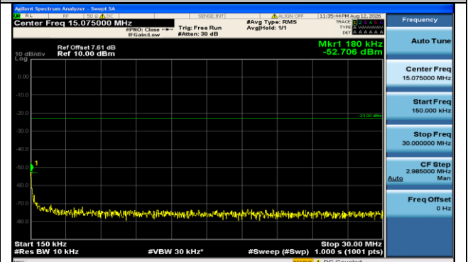
Band71-20MHz-QPSK-133222-1RB#99-0.15~30-PASS
