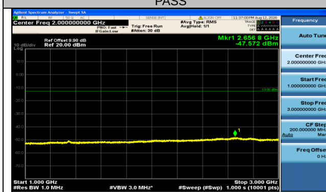
Band71-20MHz-QPSK-133222-100RB#0-1000~3000-PASS
