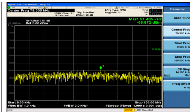
Band71-20MHz-16QAM-133222-1RB#0-0.009~0.15-PASS
