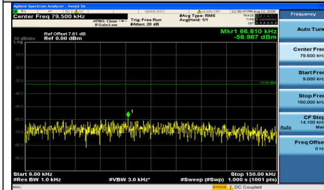
Band71-20MHz-QPSK-133222-100RB#0-0.009~0.15-PASS
