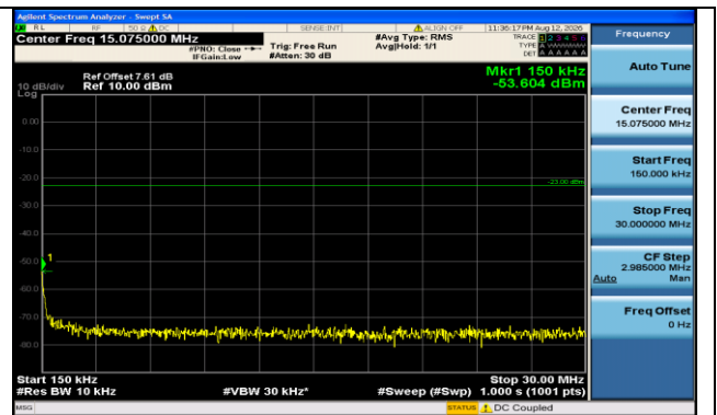
Band71-20MHz-16QAM-133222-1RB#99-0.15~30-PASS
