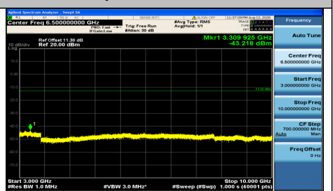
Band71-20MHz-QPSK-133222-100RB#0-3000~10000-PASS
