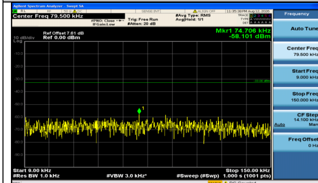
Band71-20MHz-QPSK-133222-1RB#99-0.009~0.15-PASS
