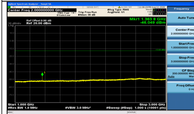
Band71-20MHz-16QAM-133222-1RB#99-1000~3000-PASS
