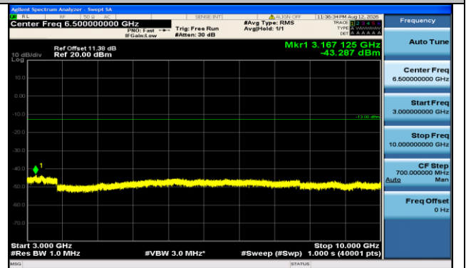
Band71-20MHz-16QAM-133222-1RB#99-3000~10000-PASS
