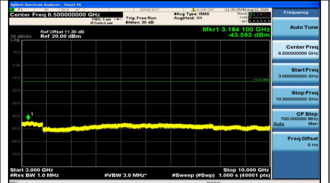
Band71-20MHz-16QAM-133222-1RB#0-3000~10000-PASS
