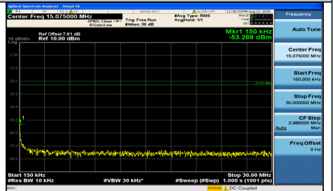
Band71-20MHz-QPSK-133222-100RB#0-0.15~30-PASS
