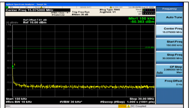
Band71-20MHz-16QAM-133222-1RB#0-0.15~30-PASS
