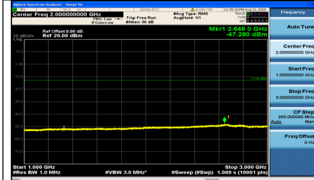
Band71-20MHz-16QAM-133222-1RB#0-1000~3000-PASS
