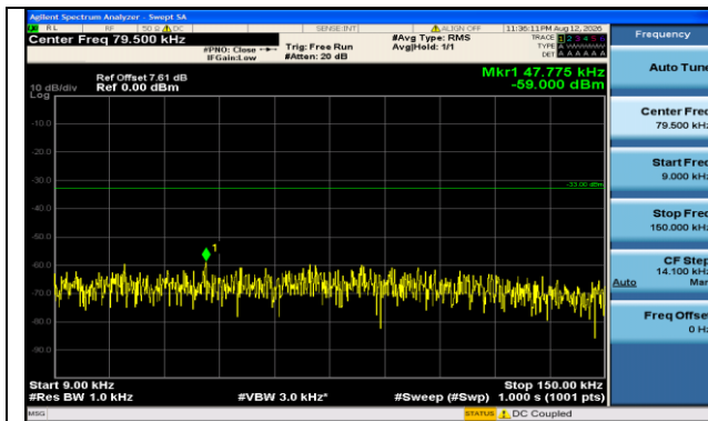
Band71-20MHz-16QAM-133222-1RB#99-0.009~0.15-PASS
