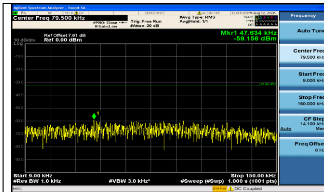
Band71-20MHz-16QAM-133222-100RB#0-0.009~0.15-PASS
