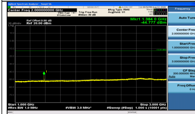
Band71-20MHz-16QAM-133322-1RB#99-1000~3000-PASS
