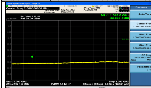
Band71-20MHz-QPSK-133322-1RB#0-1000~3000-PASS
