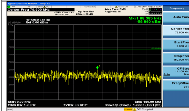
Band71-20MHz-QPSK-133322-100RB#0-0.009~0.15-PASS
