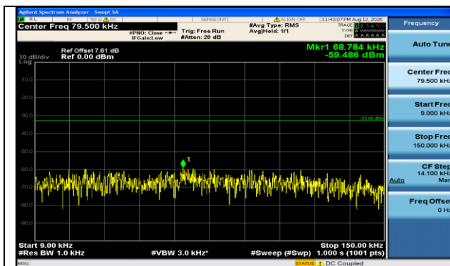
Band71-20MHz-16QAM-133372-1RB#99-0.009~0.15-PASS
