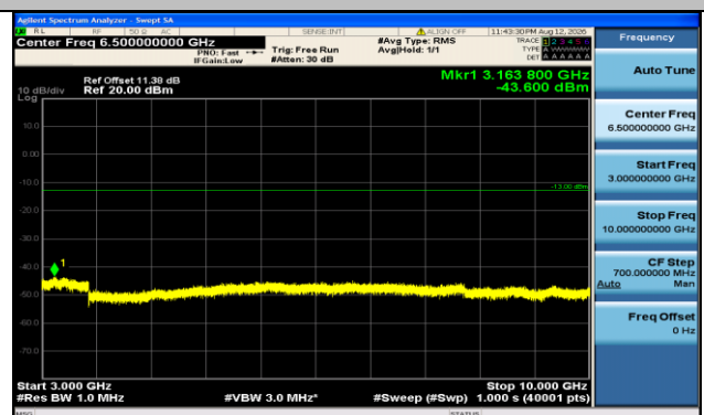
Band71-20MHz-16QAM-133372-1RB#99-3000~10000-PASS
