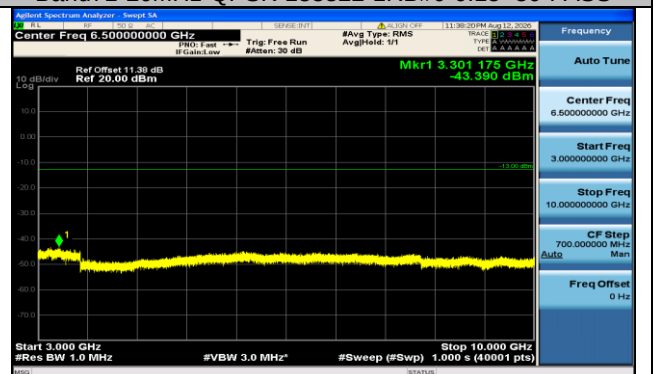
Band71-20MHz-QPSK-133322-1RB#0-3000~10000-PASS
