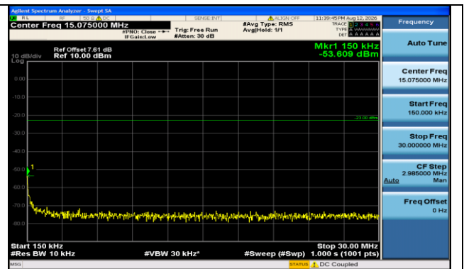
Band71-20MHz-16QAM-133322-1RB#99-0.15~30-PASS
