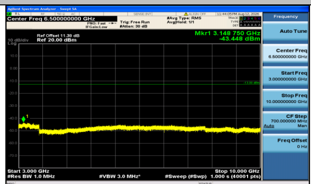
Band71-20MHz-QPSK-133372-100RB#0-3000~10000-PASS
