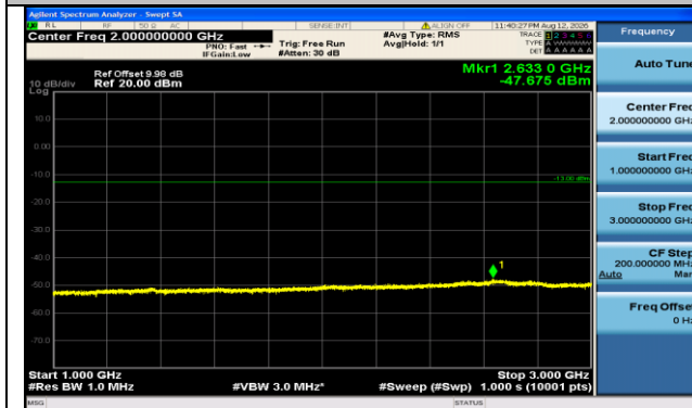
Band71-20MHz-QPSK-133322-100RB#0-1000~3000-PASS
