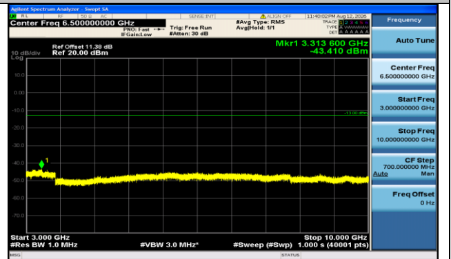
Band71-20MHz-16QAM-133322-1RB#99-3000~10000-PASS
