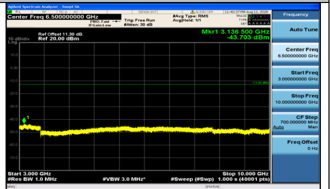
Band71-20MHz-QPSK-133322-100RB#0-3000~10000-PASS
