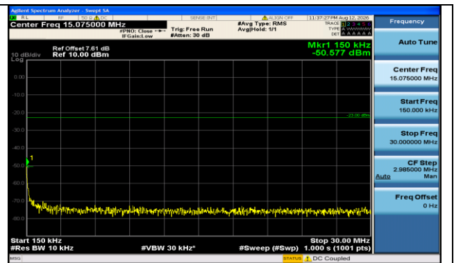
Band71-20MHz-16QAM-133222-100RB#0-0.15~30-PASS
