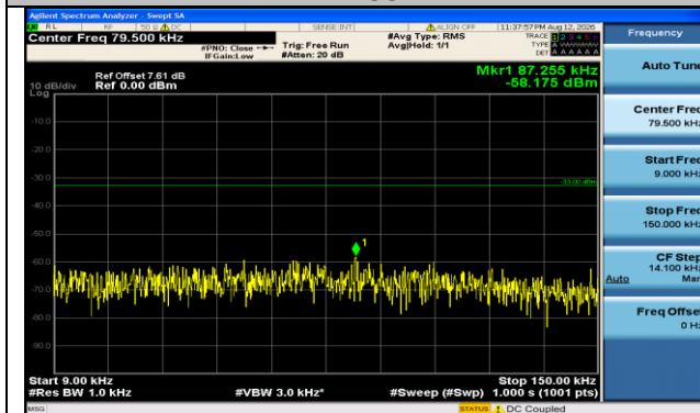
Band71-20MHz-QPSK-133322-1RB#0-0.009~0.15-PASS
