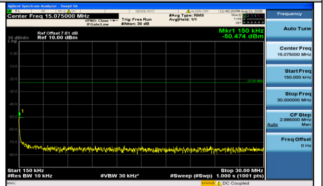
Band71-20MHz-QPSK-133322-100RB#0-0.15~30-PASS
