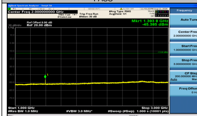
Band71-20MHz-16QAM-133372-1RB#99-1000~3000-PASS
