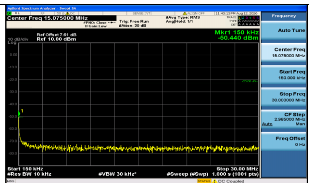
Band71-20MHz-16QAM-133372-1RB#99-0.15~30-PASS
