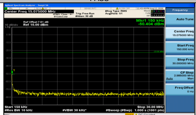
Band71-20MHz-OPSK-133372-100RB#0-0.15~30-PASS
