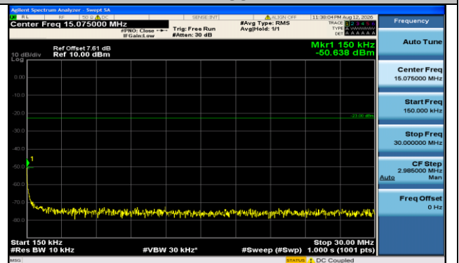
Band71-20MHz-QPSK-133322-1RB#0-0.15~30-PASS
