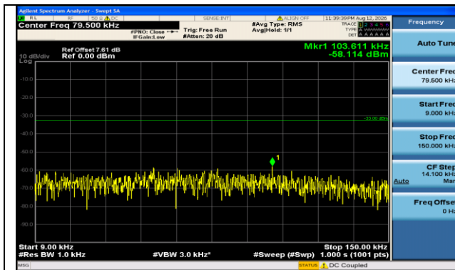
Band71-20MHz-16QAM-133322-1RB#99-0.009~0.15-PASS
