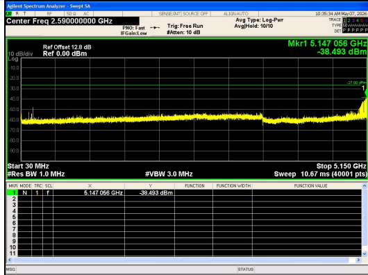
Spurious Emission:30.0~5150 MHz IEEE 802.11a_Channel 56_20MHz_Antenna 0
