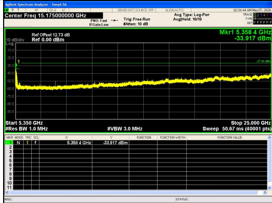
Spurious Emission:5350~25000.0 MHz IEEE 802.11a_Channel 52_20MHz_Antenna 0
