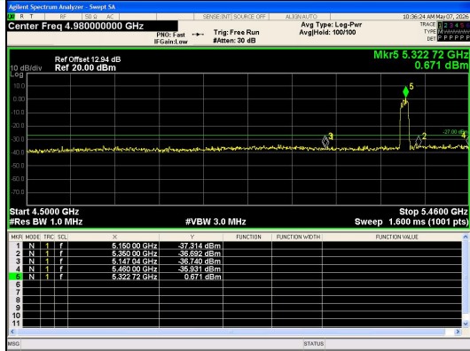
Out Of Band Emission IEEE 802.11a_Channel 64_20MHz_Antenna 0
