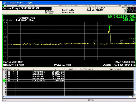
Out Of Band Emission IEEE 802.11a_Channel 52_20MHz_Antenna 0
