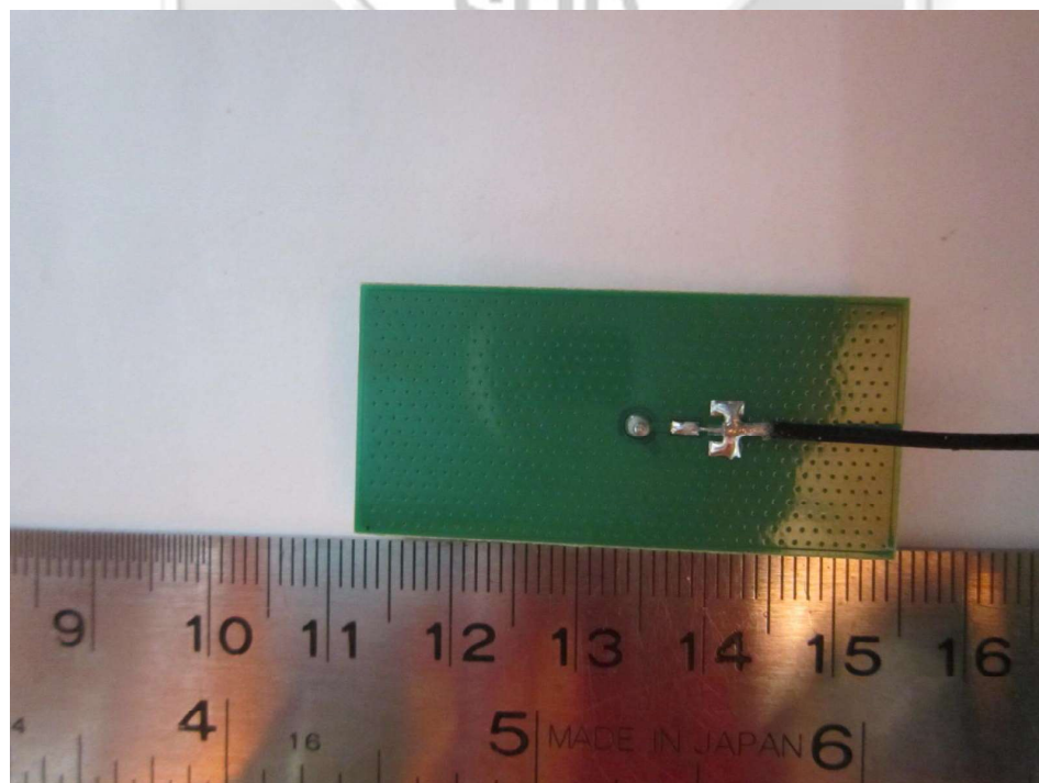
GPS Antenna Board PCB Trace Side
