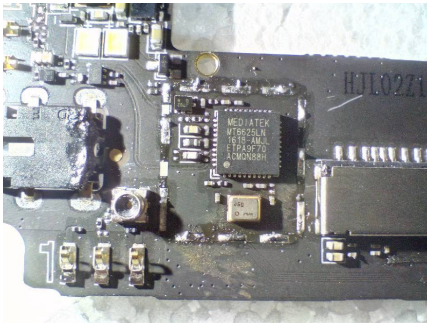
EUT – IC Chip View 4 (BT/WIFI)
