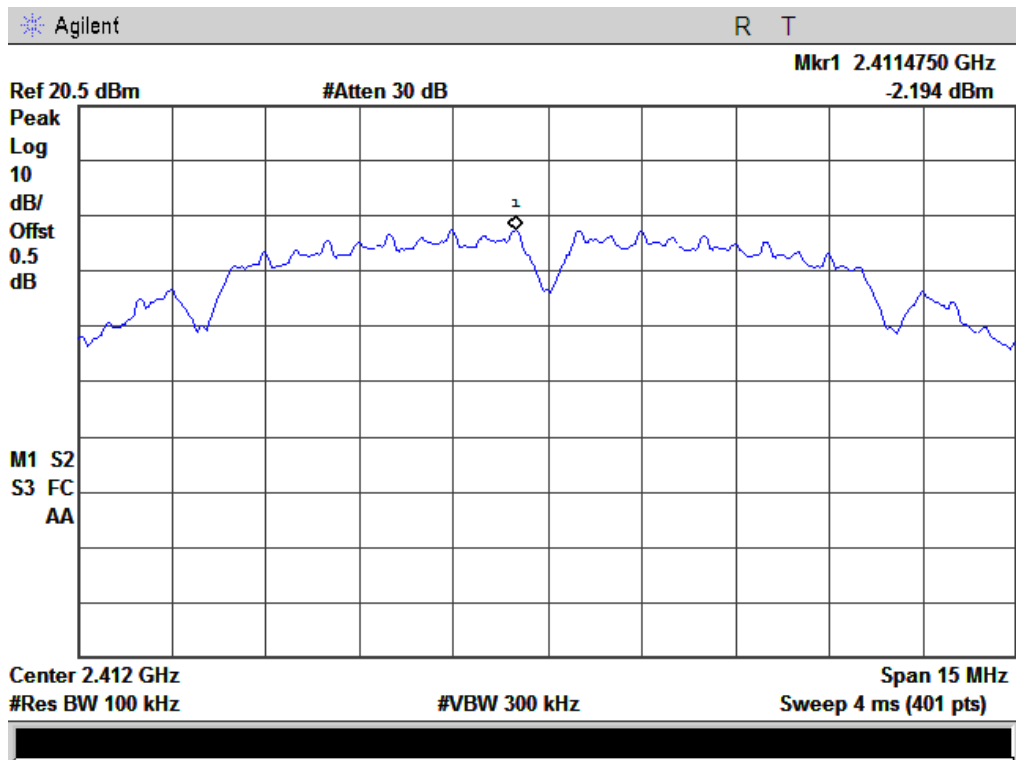
Power Spectral Density, 802.11b Low Channel
