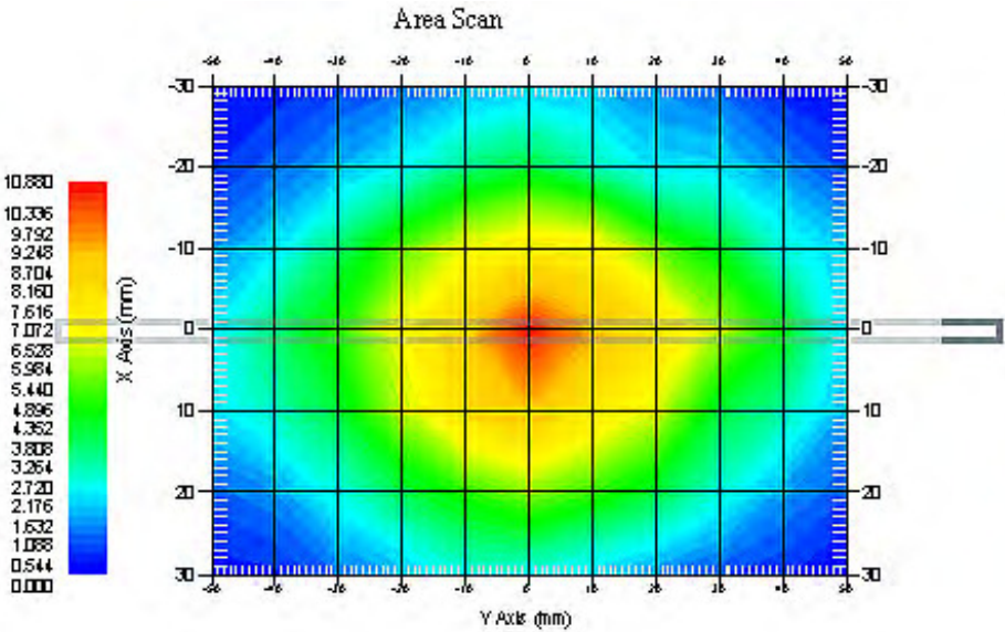
835 MHz System Validation with Head Tissue
