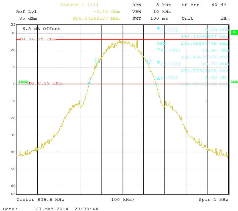
99% Occupied Emissions Bandwidth & 26 dB Emissions Bandwidth
