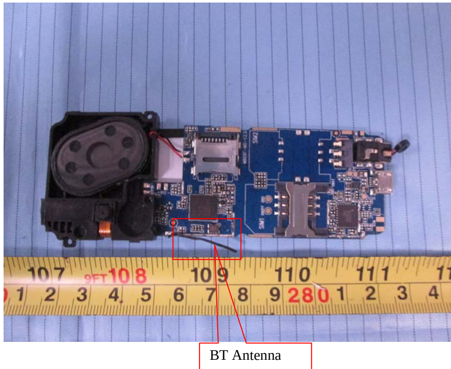
EUT – Main Board Bottom Shielding Off View
