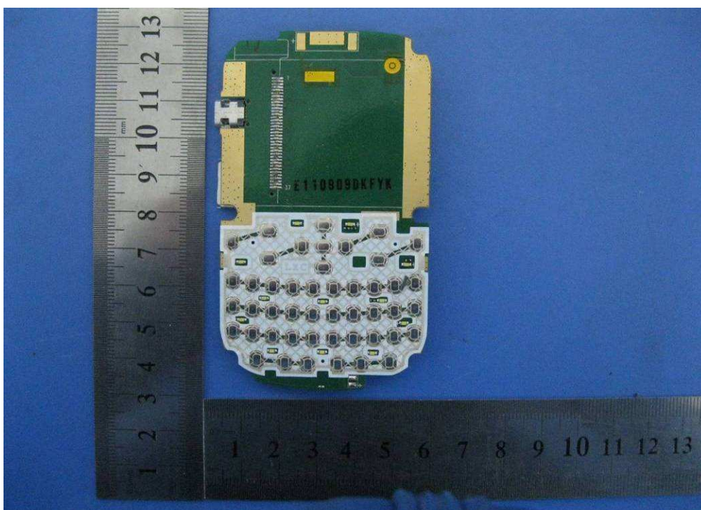
EUT – Main Board Shielding off Bottom View
