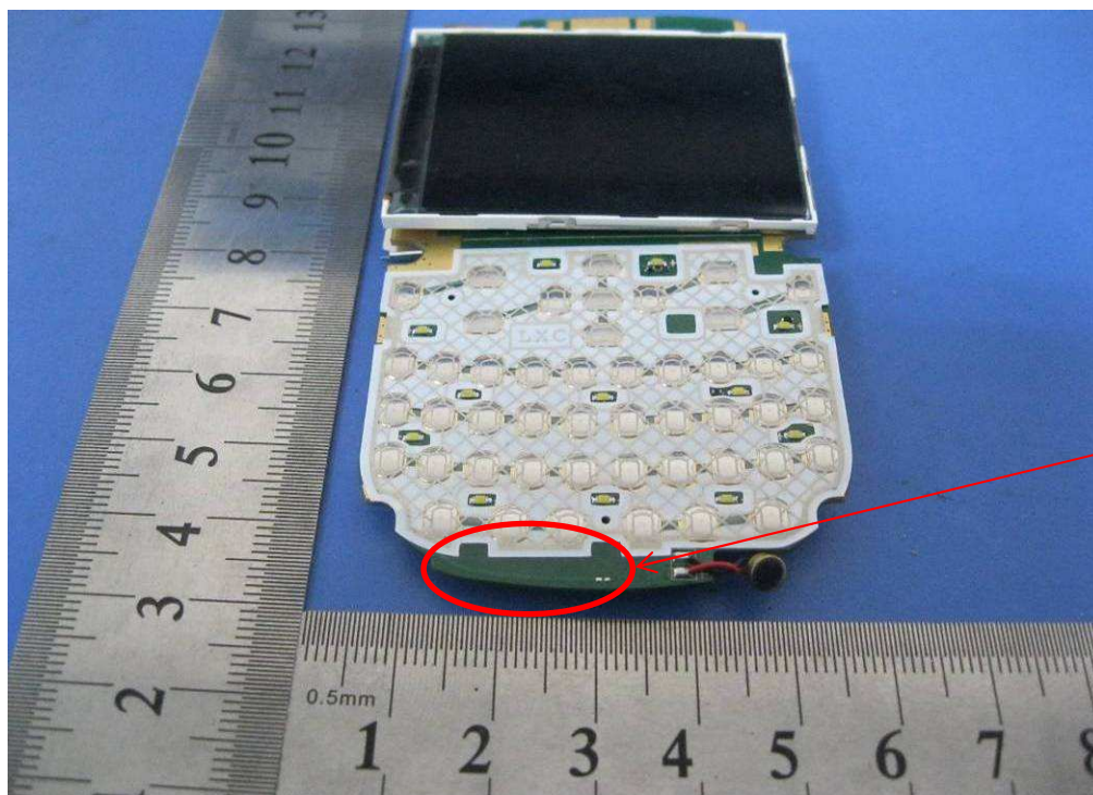
Bluetooth Antenna - Top View
