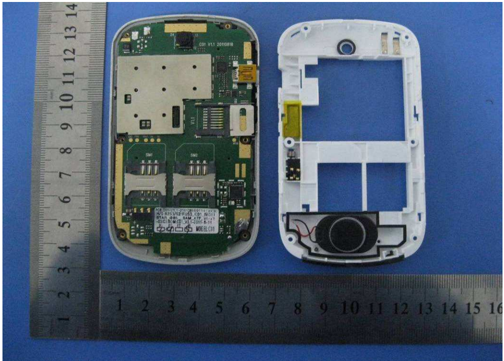
EUT –Rear Cover off View
