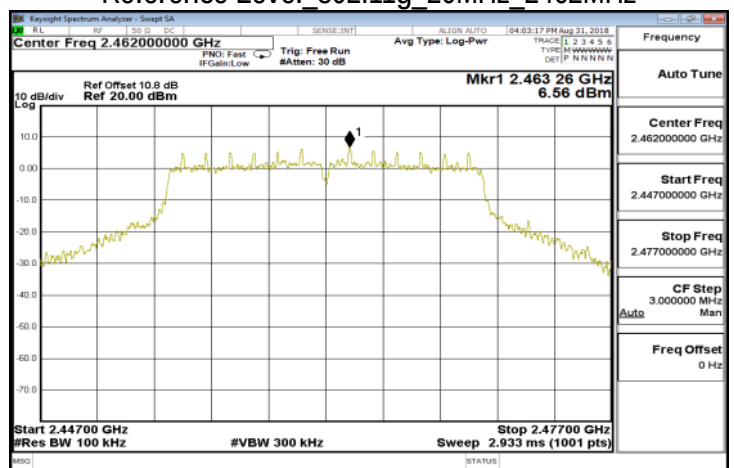
Reference Level 802.11g 20MHz 2462MHz
