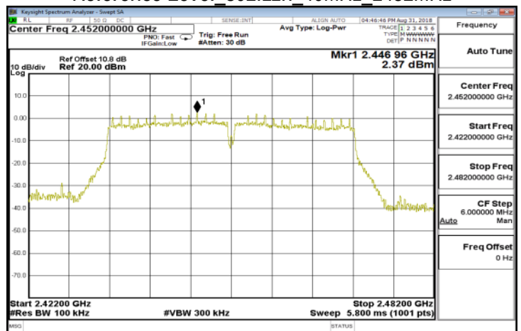
Reference Level 802.11n 40MHz 2452MHz
