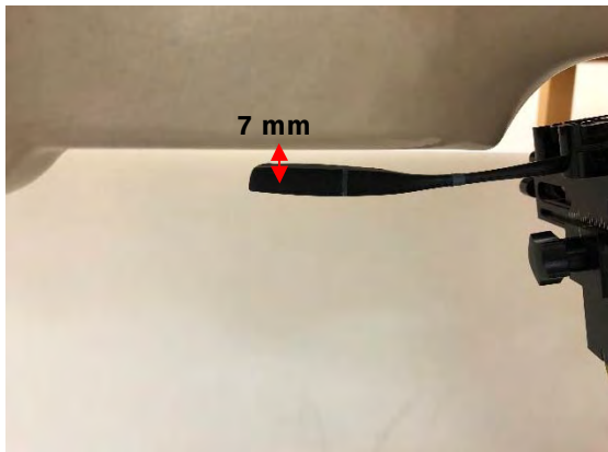
Fig.3 EUT inner surface to flat phantom
