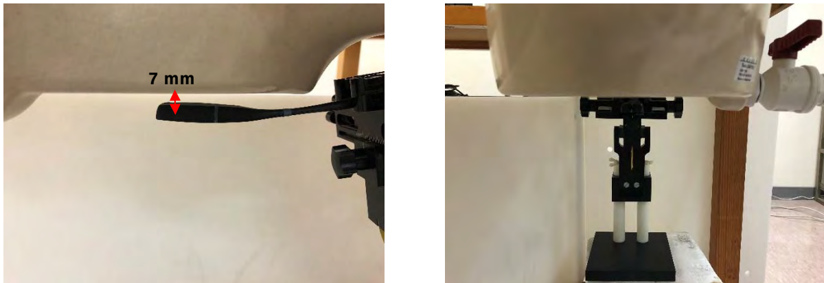
Fig.3 EUT inner surface to flat phantom
