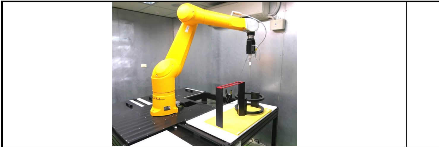
Fig-3.3 DASY5 Measurement System
