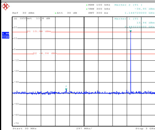
CSE Plot on CH 78 between 30 MHz ~ 3 GHz
