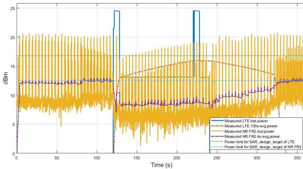
Figure 8.3-1 Conducted power of LTE B2 and radiated EIRP of FR2 n261 in EN-DC max power case
