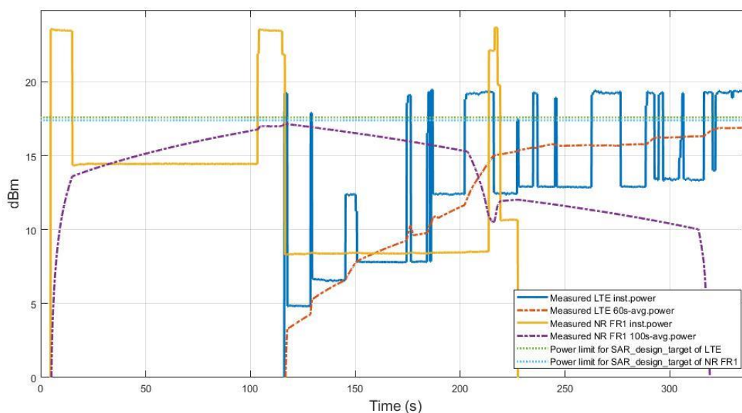
Figure 7.8-1 Time average SAR of LTE B48 and FR1 n25 in EN-DC case
