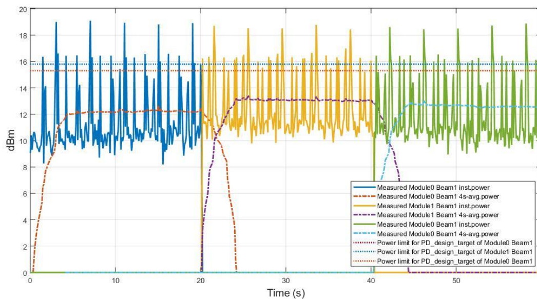
Figure 8.4-1 Measured radiated EIRP of FR2 n260 in mmWave Module beam change case TC03
