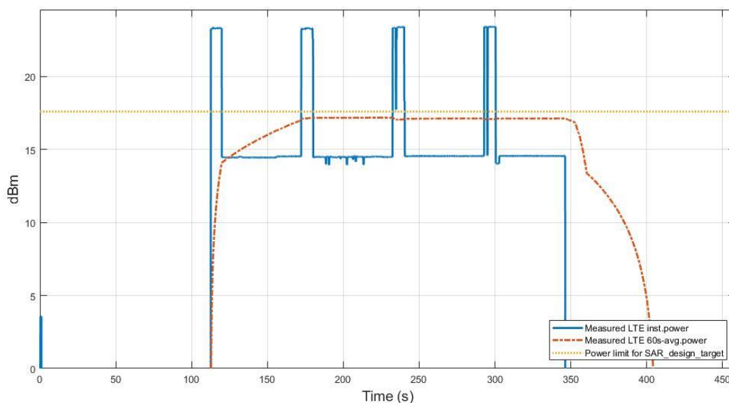
Figure 7.10-1 Conducted transmitted power of LTE Band 7 in UL CA
