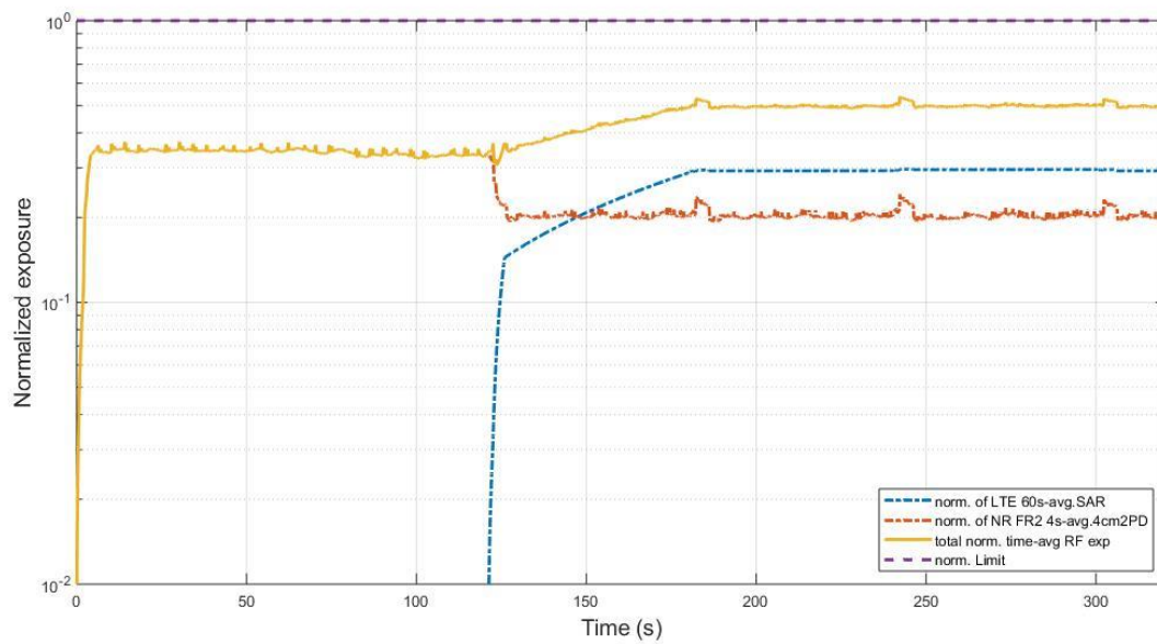
Figure 8.2-2 Total normalized time-average RF exposure in TC01
