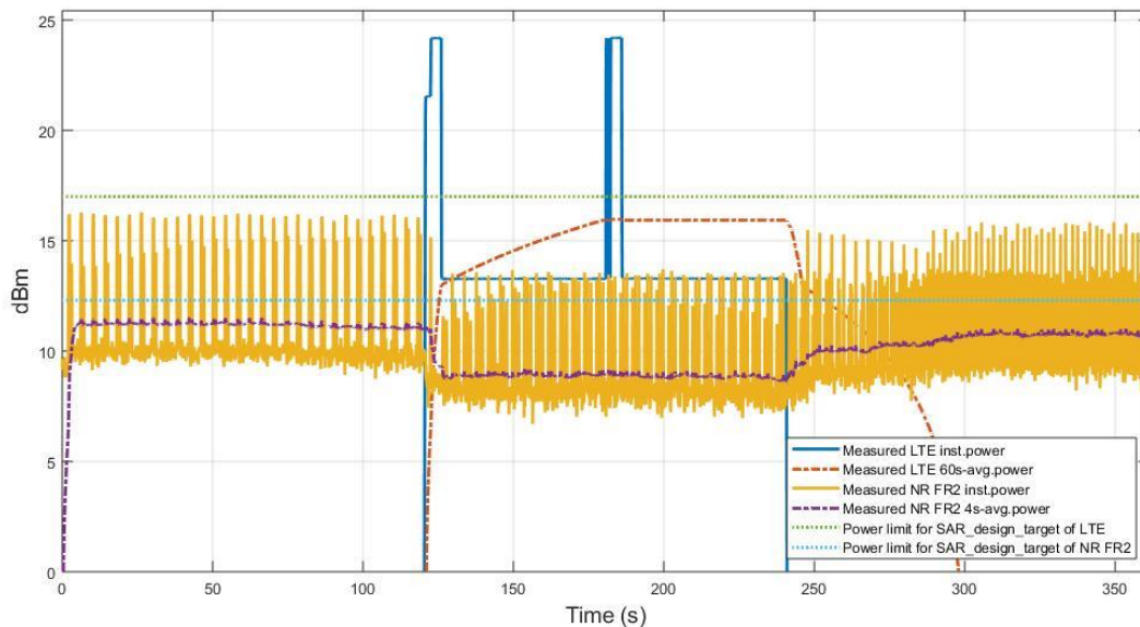
Figure 8.3-1 Conducted power of LTE B2 and radiated EIRP of FR2 n260 in EN-DC
