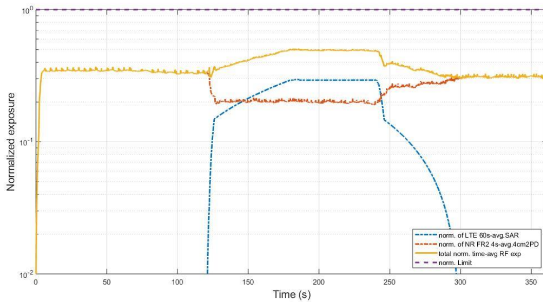
Figure 8.3-2 Total normalized time-average RF exposure in TC02
