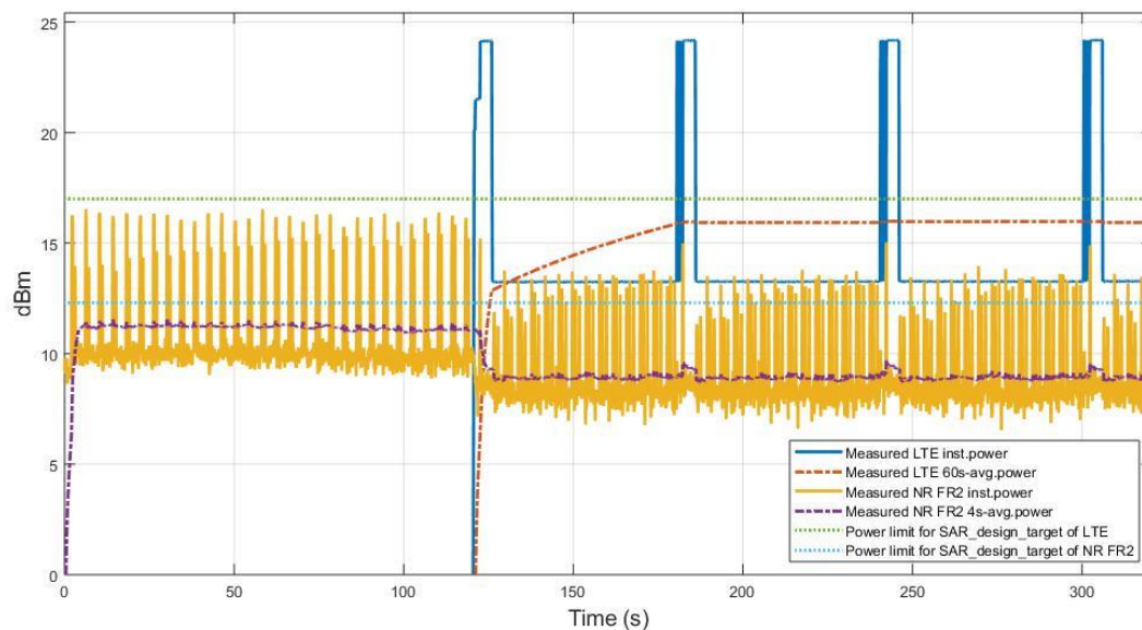
Figure 8.2-1 Conducted power of LTE B2 and radiated EIRP of FR2 n260 in EN-DC
