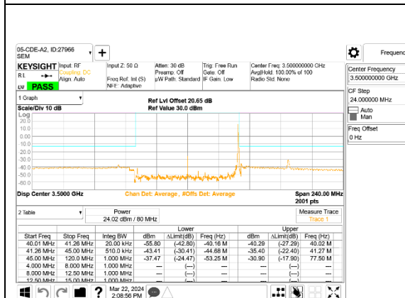
5G NR n77 80MHz BPSK Middle Channel RB1-216, ID:27966
