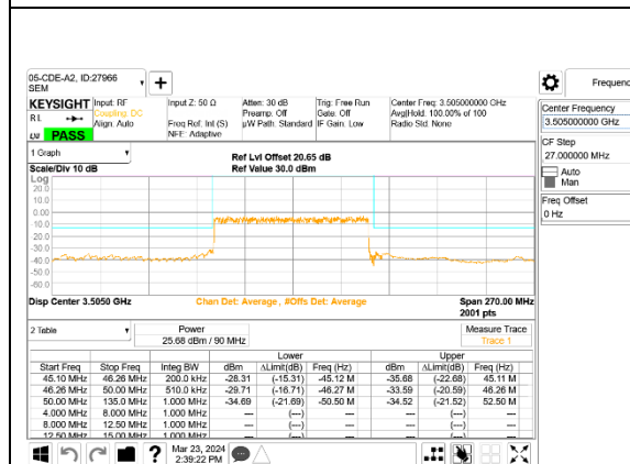
5G NR n77 90MHz BPSK High Channel RB243-0, ID:27966
