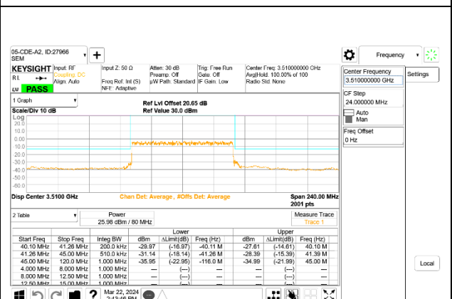
5G NR n77 80MHz BPSK High Channel RB216-0, ID:27966
