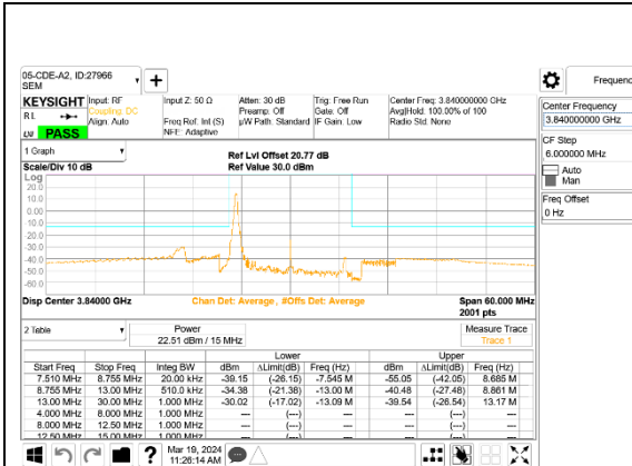
5G NR n77 15MHz BPSK Middle Channel RB1-0, ID:27966
