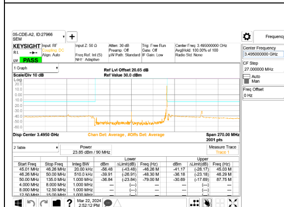
5G NR n77 90MHz BPSK Low Channel RB1-244, ID:27966
