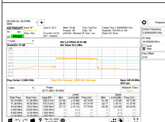
5G NR n77 80MHz BPSK Middle Channel RB216-0, ID:27966
