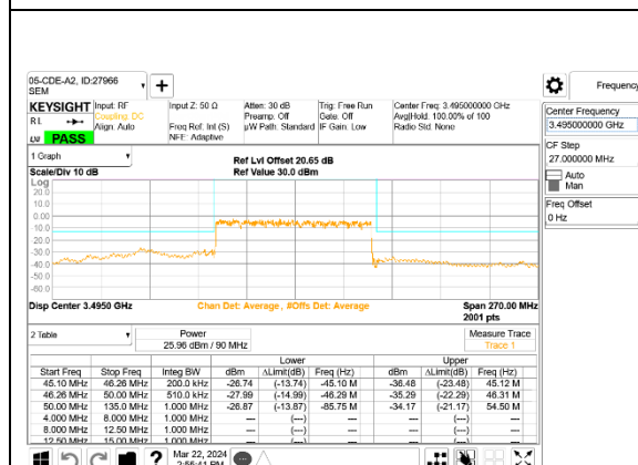
5G NR n77 90MHz BPSK Low Channel RB243-0, ID:27966
