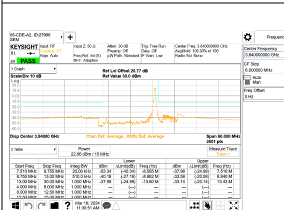
5G NR n77 15MHz BPSK Middle Channel RB1-37, ID:27966
