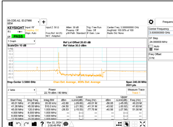
5G NR n77 80MHz BPSK Middle Channel RB1-0, ID:27966
