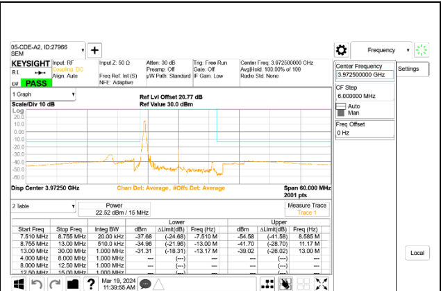
5G NR n77 15MHz BPSK High Channel RB1-0, ID:27966
