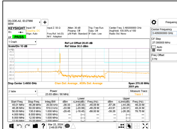
5G NR n77 90MHz BPSK Low Channel RB1-0, ID:27966
