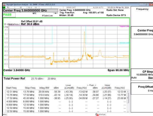
5G NR n77 25MHz BPSK Middle Channel RB1-64, ID:28498
