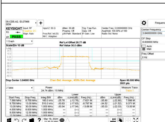
5G NR n77 15MHz BPSK Middle Channel RB36-0, ID:27966
