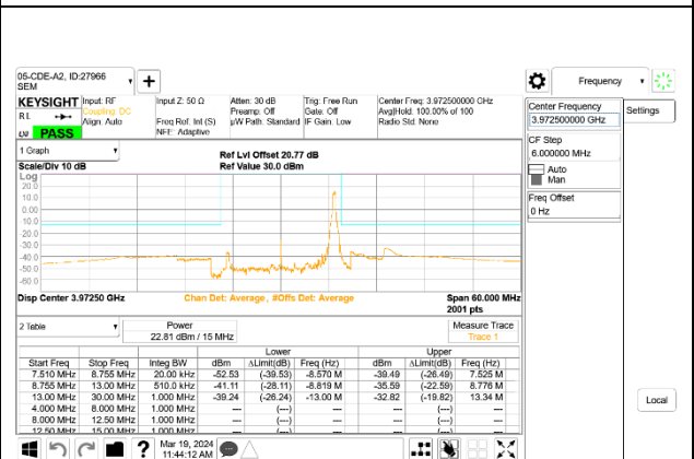
5G NR n77 15MHz BPSK High Channel RB1-37, ID:27966
