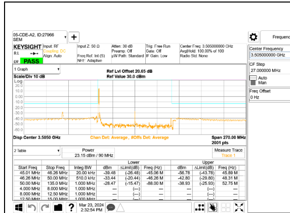
5G NR n77 90MHz BPSK High Channel RB1-0, ID:27966
