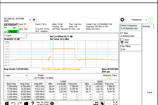
5G NR n77 15MHz BPSK High Channel RB36-0, ID:27966
