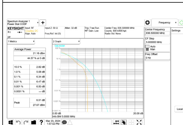
5G NR n26 15MHz BPSK Middle Channel, ID:50822
