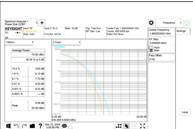
5G NR n25 35MHz 16QAM Middle Channel, ID:50822
