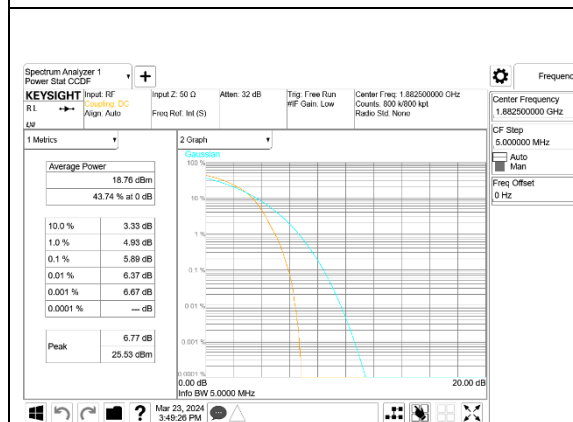
5G NR n25 25MHz BPSK Middle Channel, ID:50822
