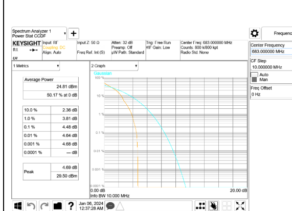
LTE B71 10MHz QPSK Middle Channel, ID:19210
