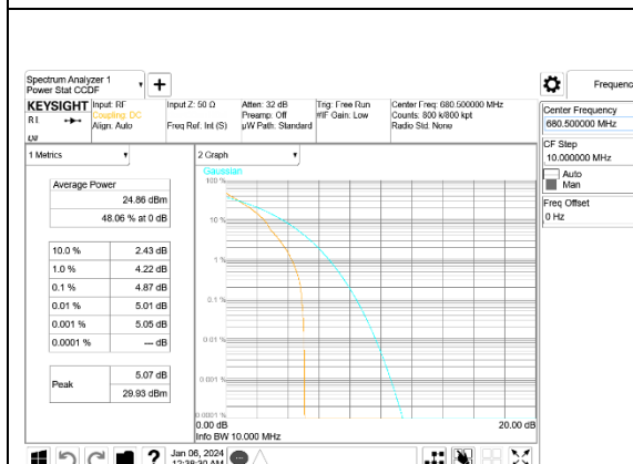
LTE B71 15MHz QPSK Middle Channel, ID:19210
