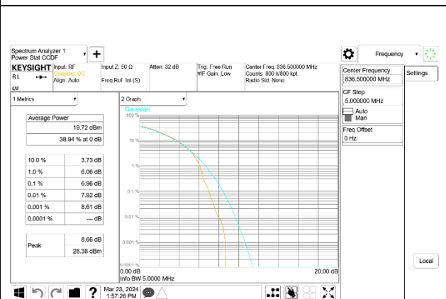
5G NR n26 15MHz 16QAM Middle Channel, ID:50822
