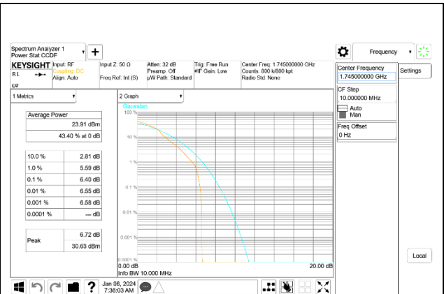
LTE B66 10MHz 16QAM Middle Channel, ID:39005
