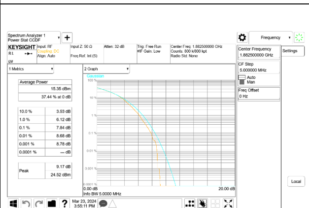
5G NR n25 40MHz 16QAM Middle Channel, ID:50822
