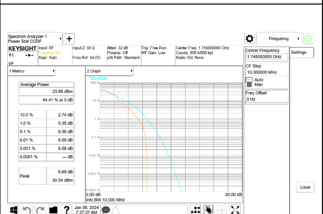
LTE B66 15MHz 16QAM Middle Channel, ID:39005
