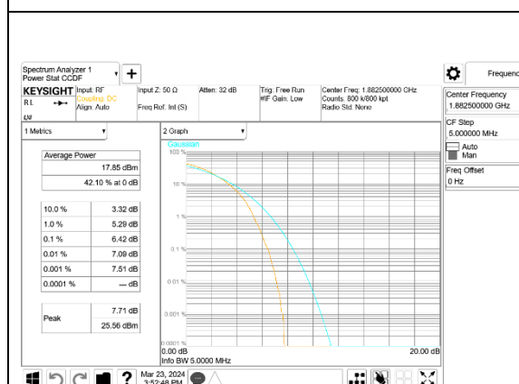
5G NR n25 30MHz BPSK Middle Channel, ID:50822
