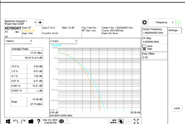
5G NR n25 25MHz 16QAM Middle Channel, ID:50822
