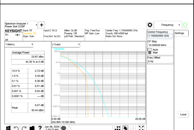
LTE B66 20MHz 16QAM Middle Channel, ID:39005
