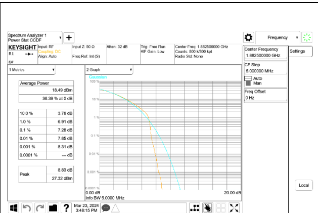
5G NR n25 20MHz 16QAM Middle Channel, ID:50822
