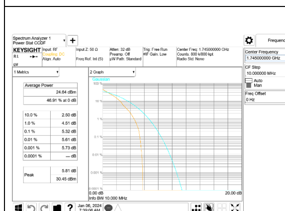
LTE B66 20MHz QPSK Middle Channel, ID:39005
