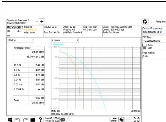
LTE B71 5MHz QPSK Middle Channel, ID:19210
