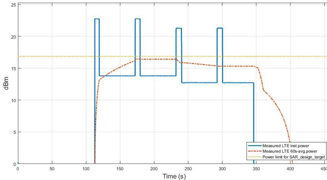
Figure 7.9-1 Conducted transmitted power of LTE Band 5 in UL CA
