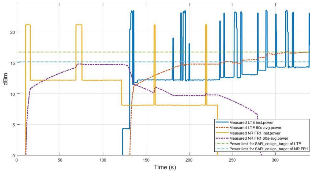
Figure 7.6-1 Time average SAR of LTE B66 and FR1 n77 in EN-DC case
