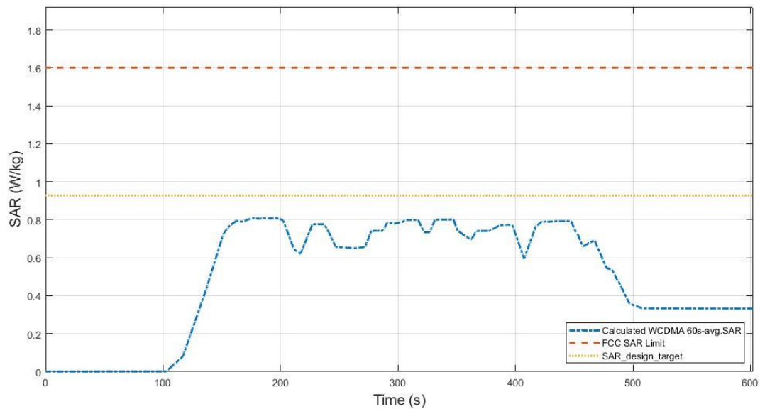
Figure 7.3-16 Total time-averaged SAR
