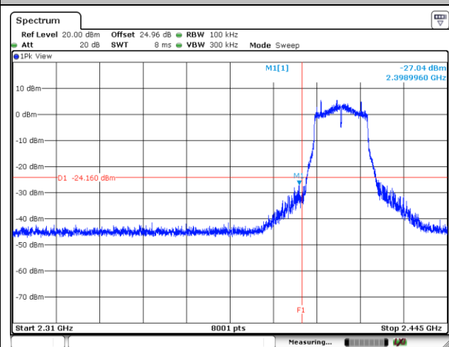
Channel 01 Plot
