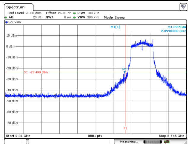
Channel 01 Plot
