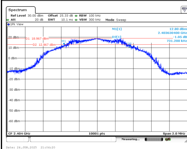
6 dB Bandwidth Plot on Channel 02
