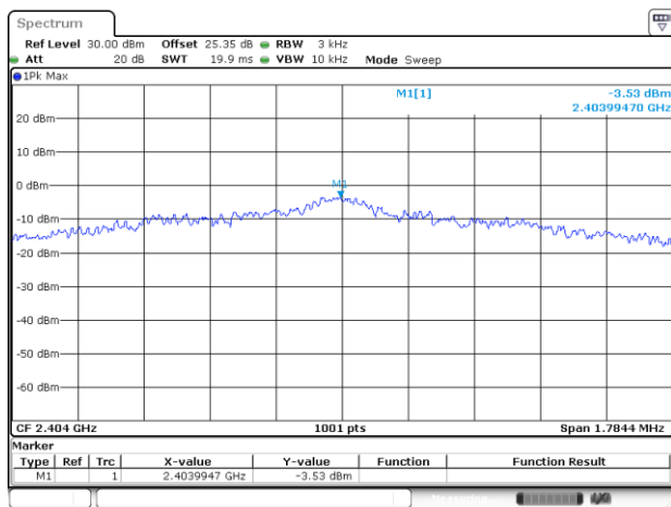
Power Density (dBm/3kHz) Plot Channel 02
