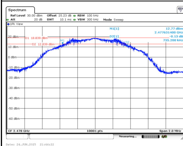
6 dB Bandwidth Plot on Channel 76
