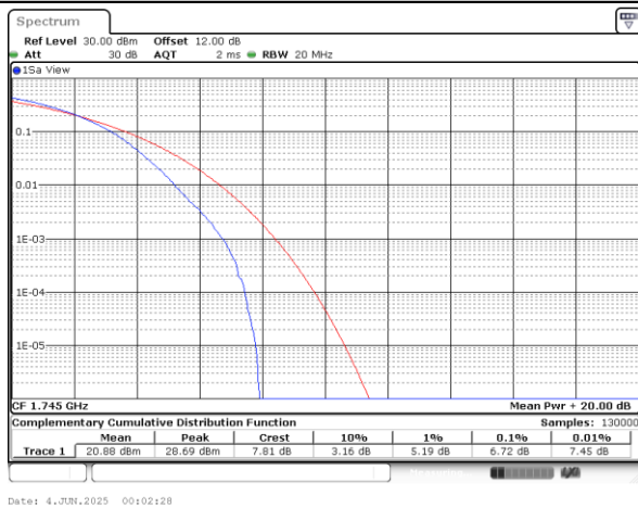
LTE Band 66 / 20MHz / 64QAM
